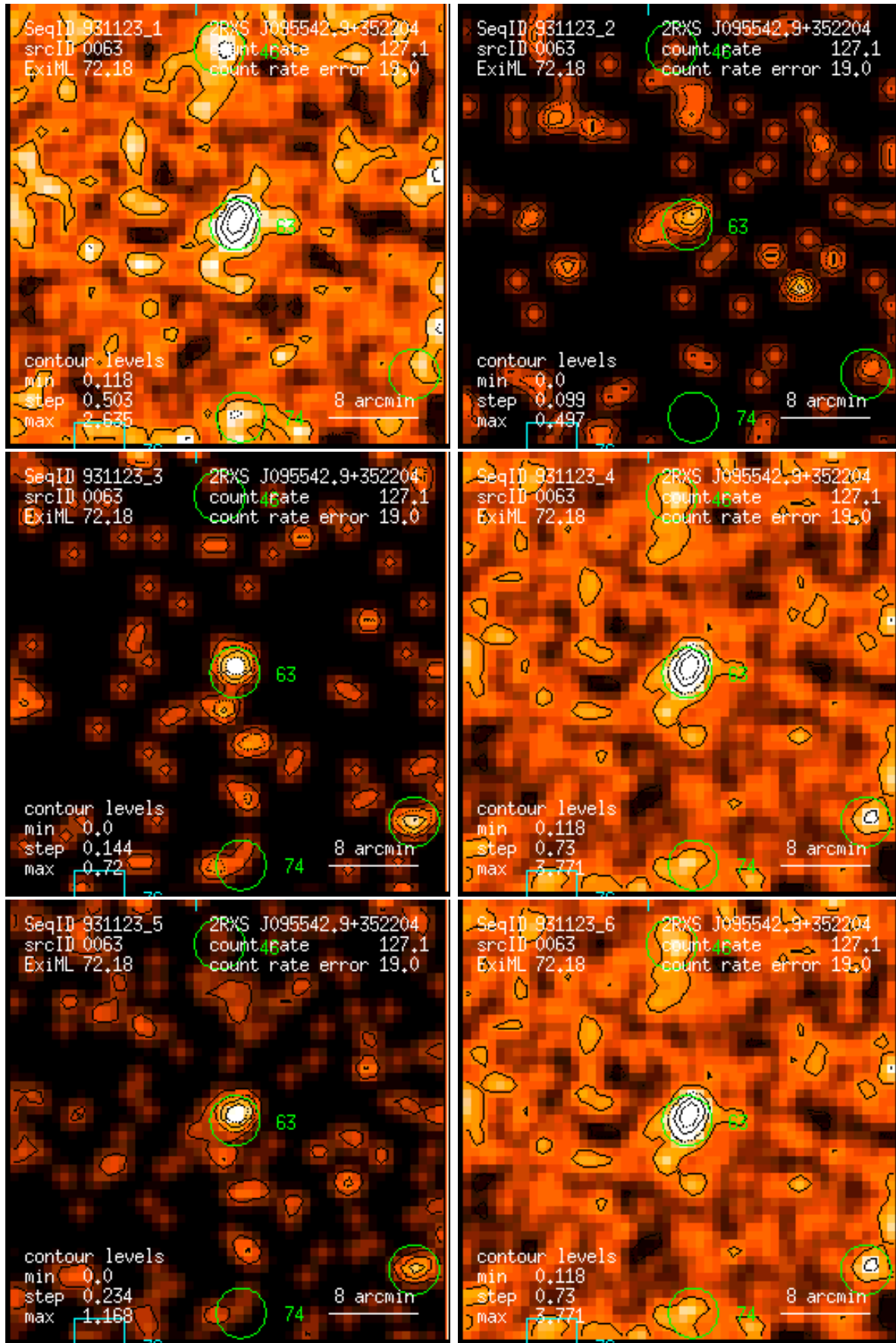
Figure 63: RASS 931123: detection 0063: band rate images, Gaussian filter: (1) PSPC channels 11 – 41, (2) 52 – 90, (3) 91 – 201, (4) 11 – 235, (5) 52 – 201, (6) 11 – 201. Broad band rates in counts/ks. Band rate contour levels in counts/ks/arcmin 2 .
