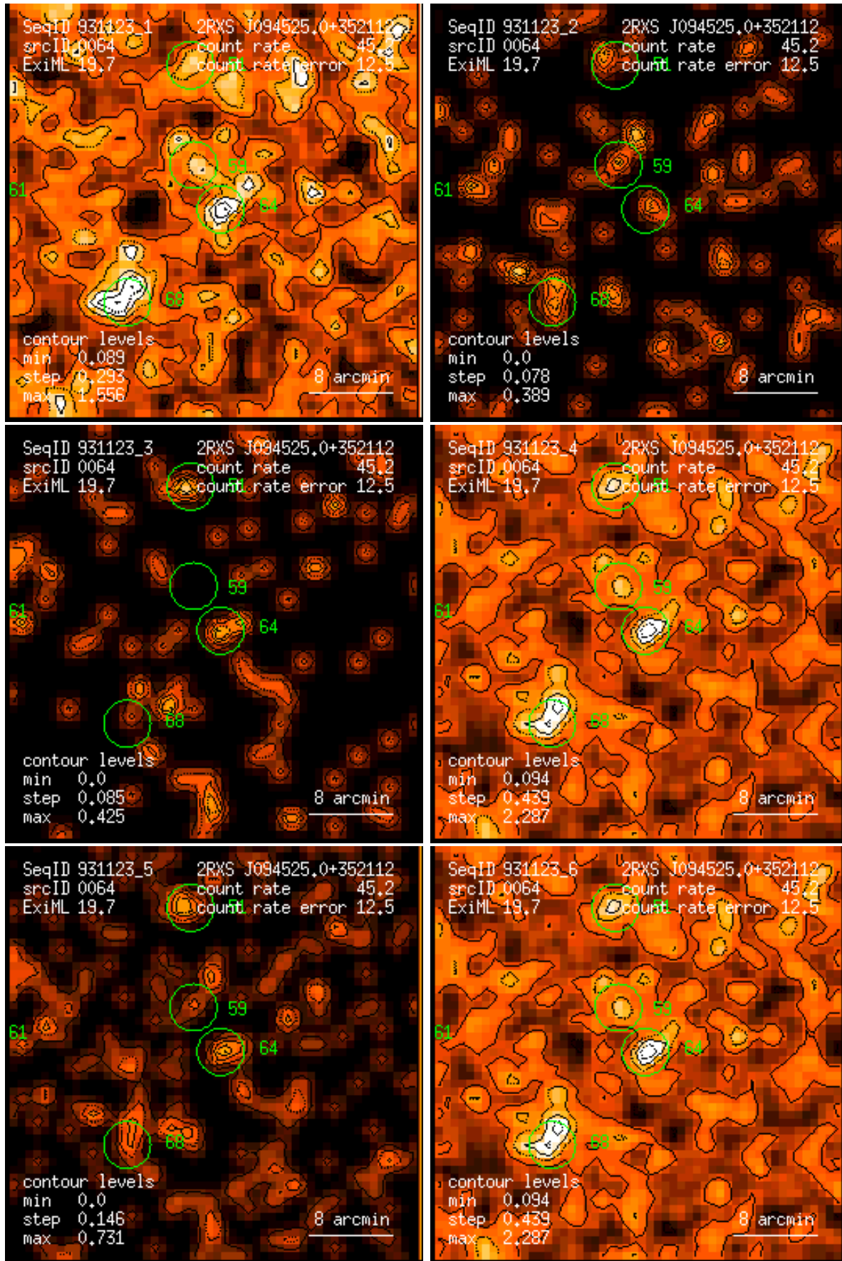
Figure 64: RASS 931123: detection 0064: band rate images, Gaussian filter: (1) PSPC channels 11 – 41, (2) 52 – 90, (3) 91 – 201, (4) 11 – 235, (5) 52 – 201, (6) 11 – 201. Broad band rates in counts/ks. Band rate contour levels in counts/ks/arcmin 2 .
