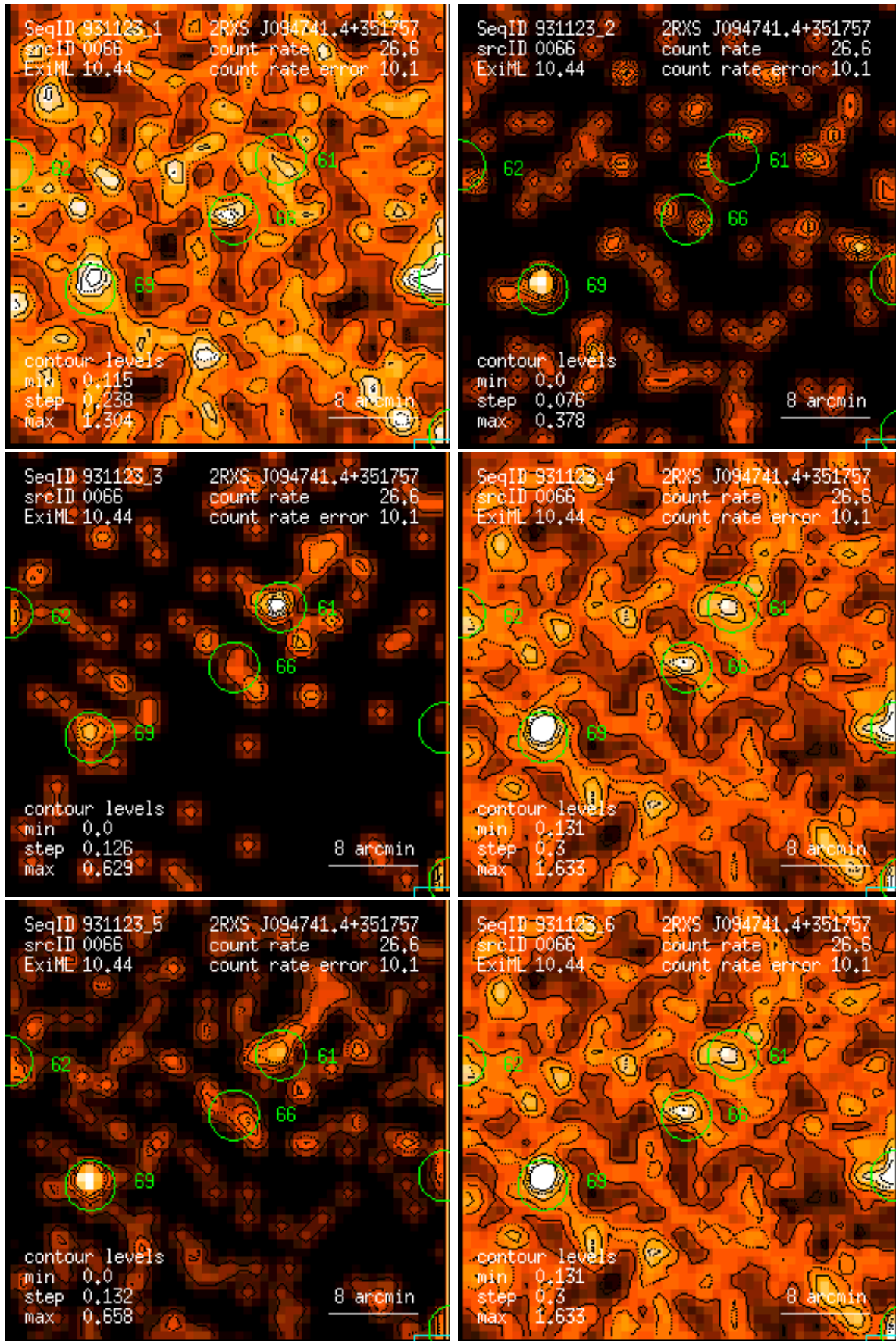
Figure 66: RASS 931123: detection 0066: band rate images, Gaussian filter: (1) PSPC channels 11 – 41, (2) 52 – 90, (3) 91 – 201, (4) 11 – 235, (5) 52 – 201, (6) 11 – 201. Broad band rates in counts/ks. Band rate contour levels in counts/ks/arcmin 2 .
