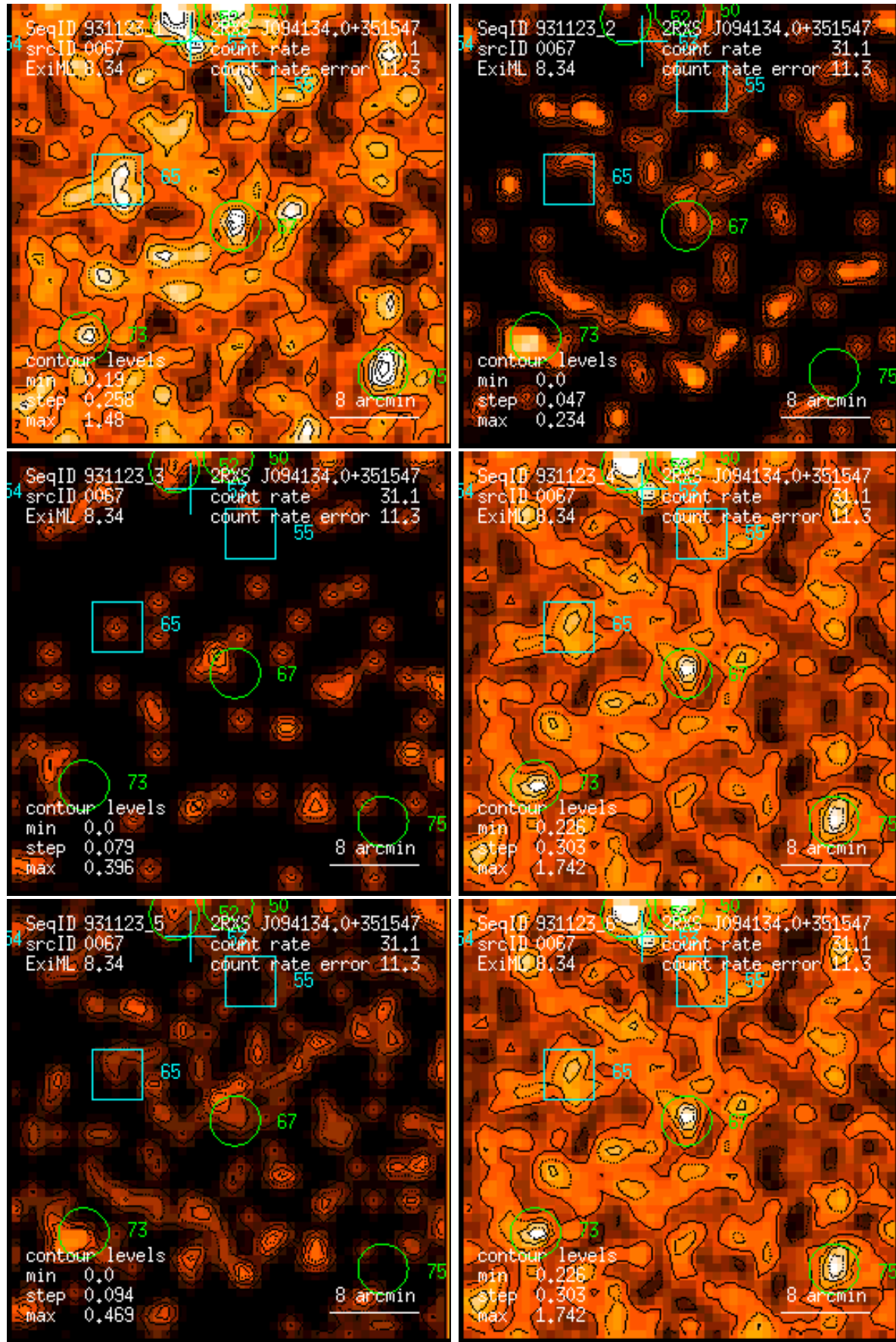
Figure 67: RASS 931123: detection 0067: band rate images, Gaussian filter: (1) PSPC channels 11 – 41, (2) 52 – 90, (3) 91 – 201, (4) 11 – 235, (5) 52 – 201, (6) 11 – 201. Broad band rates in counts/ks. Band rate contour levels in counts/ks/arcmin 2 .
