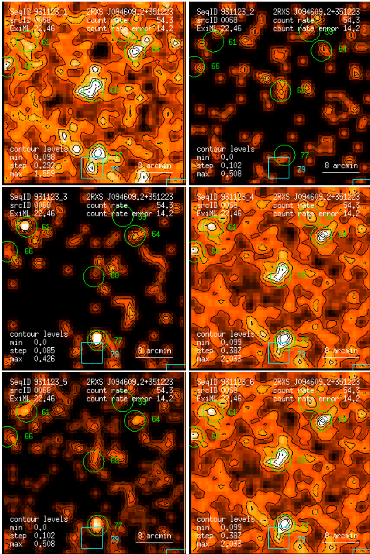
Figure 68: RASS 931123: detection 0068: band rate images, Gaussian filter: (1) PSPC channels 11 – 41, (2) 52 – 90, (3) 91 – 201, (4) 11 – 235, (5) 52 – 201, (6) 11 – 201. Broad band rates in counts/ks. Band rate contour levels in counts/ks/arcmin 2 .
