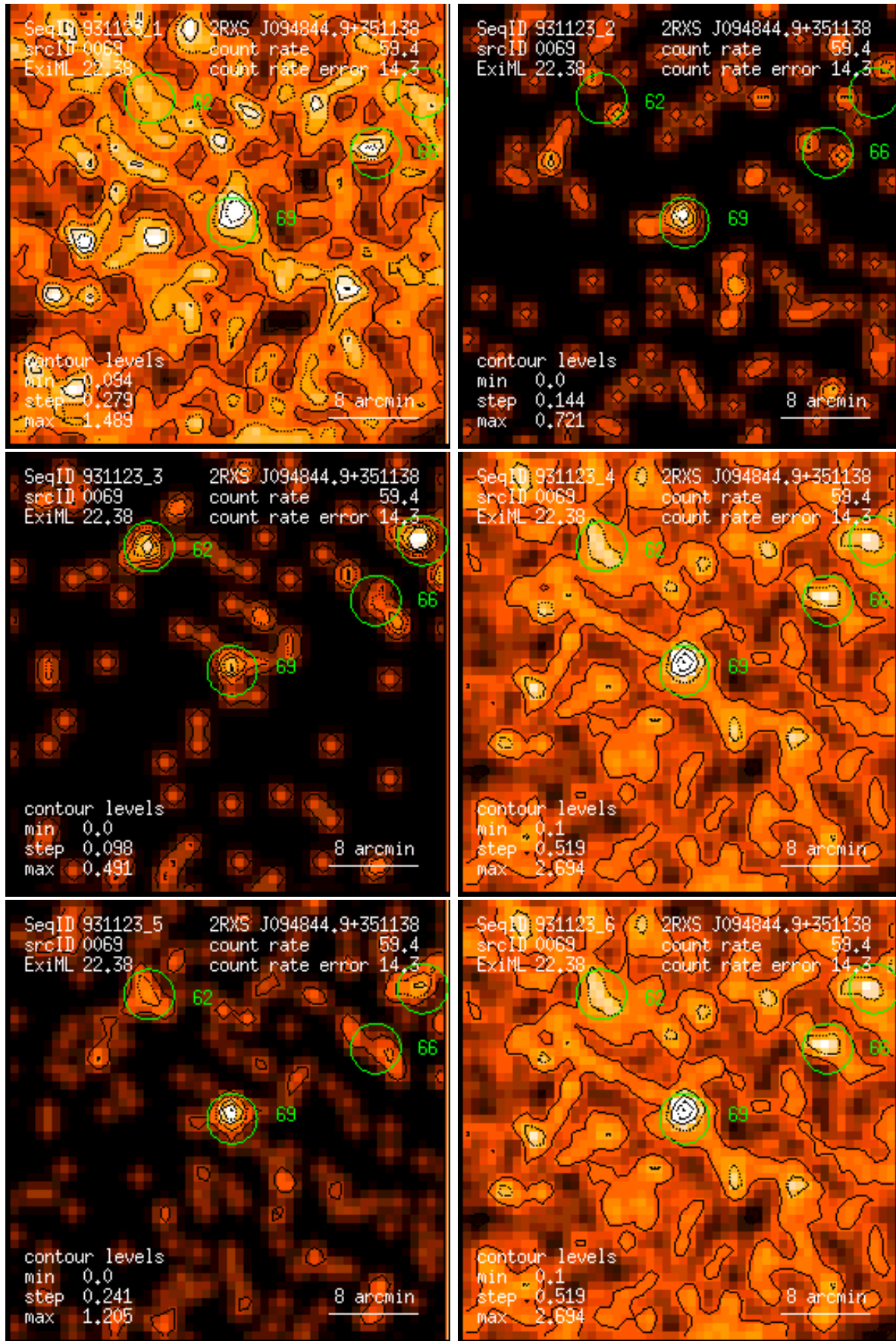
Figure 69: RASS 931123: detection 0069: band rate images, Gaussian filter: (1) PSPC channels 11 – 41, (2) 52 – 90, (3) 91 – 201, (4) 11 – 235, (5) 52 – 201, (6) 11 – 201. Broad band rates in counts/ks. Band rate contour levels in counts/ks/arcmin 2 .
