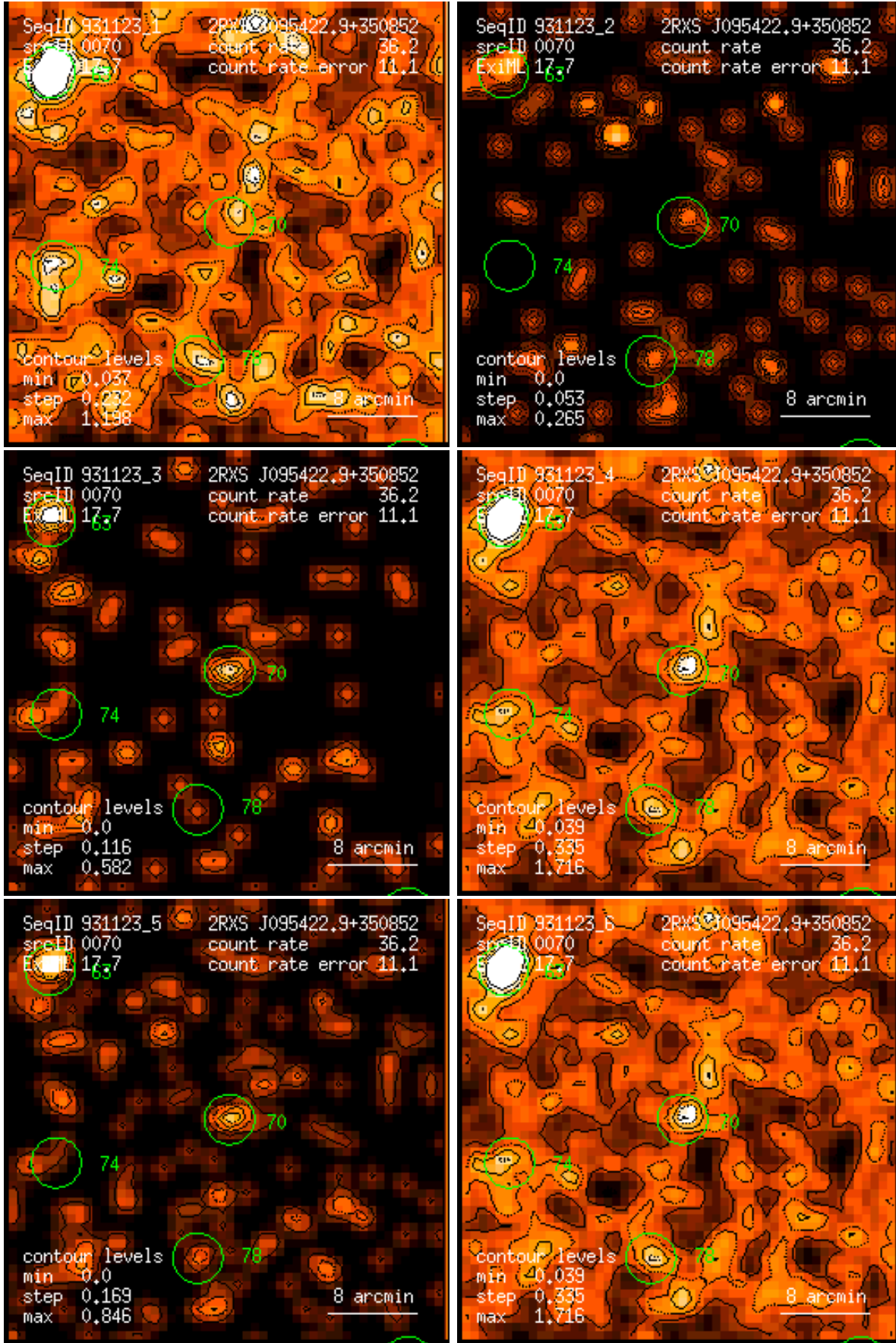
Figure 70: RASS 931123: detection 0070: band rate images, Gaussian filter: (1) PSPC channels 11 – 41, (2) 52 – 90, (3) 91 – 201, (4) 11 – 235, (5) 52 – 201, (6) 11 – 201. Broad band rates in counts/ks. Band rate contour levels in counts/ks/arcmin 2 .
