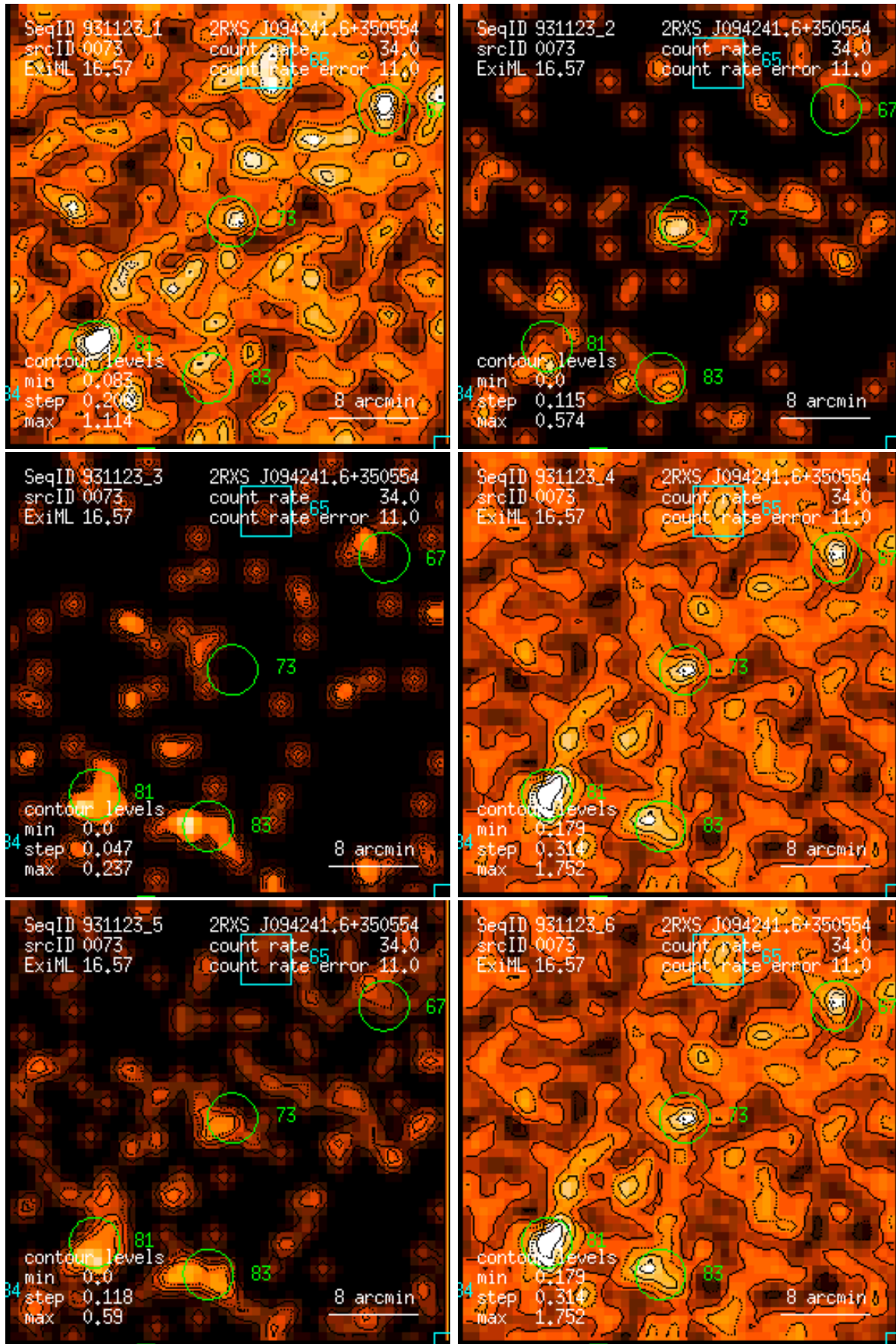
Figure 73: RASS 931123: detection 0073: band rate images, Gaussian filter: (1) PSPC channels 11 – 41, (2) 52 – 90, (3) 91 – 201, (4) 11 – 235, (5) 52 – 201, (6) 11 – 201. Broad band rates in counts/ks. Band rate contour levels in counts/ks/arcmin 2 .
