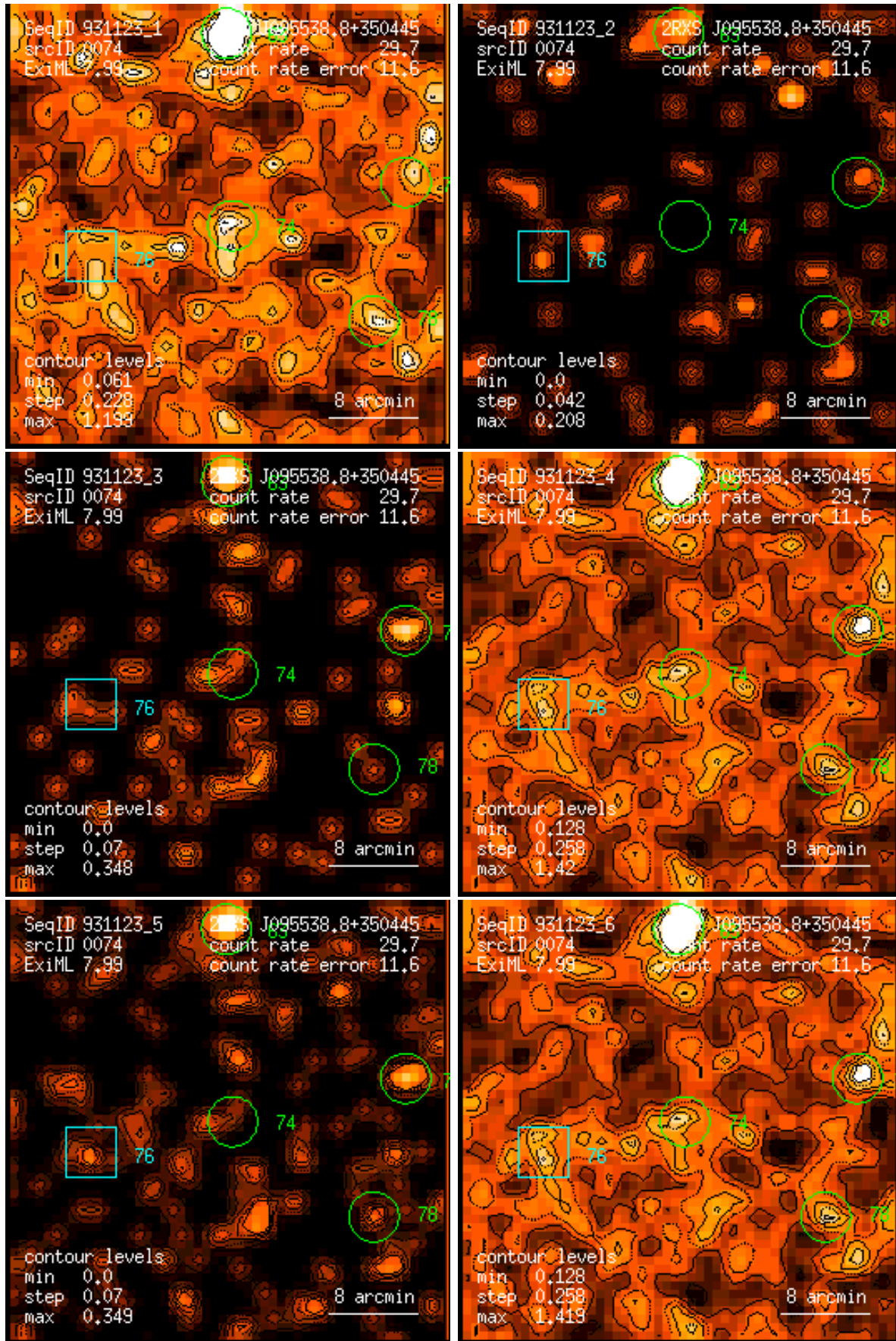
Figure 74: RASS 931123: detection 0074: band rate images, Gaussian filter: (1) PSPC channels 11 – 41, (2) 52 – 90, (3) 91 – 201, (4) 11 – 235, (5) 52 – 201, (6) 11 – 201. Broad band rates in counts/ks. Band rate contour levels in counts/ks/arcmin 2 .
