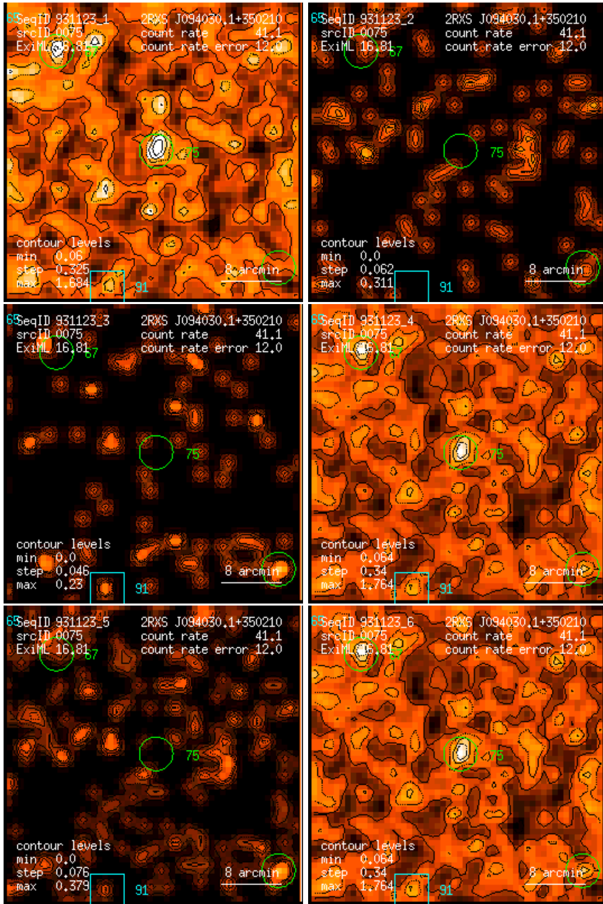
Figure 75: RASS 931123: detection 0075: band rate images, Gaussian filter: (1) PSPC channels 11 – 41, (2) 52 – 90, (3) 91 – 201, (4) 11 – 235, (5) 52 – 201, (6) 11 – 201. Broad band rates in counts/ks. Band rate contour levels in counts/ks/arcmin 2 .
