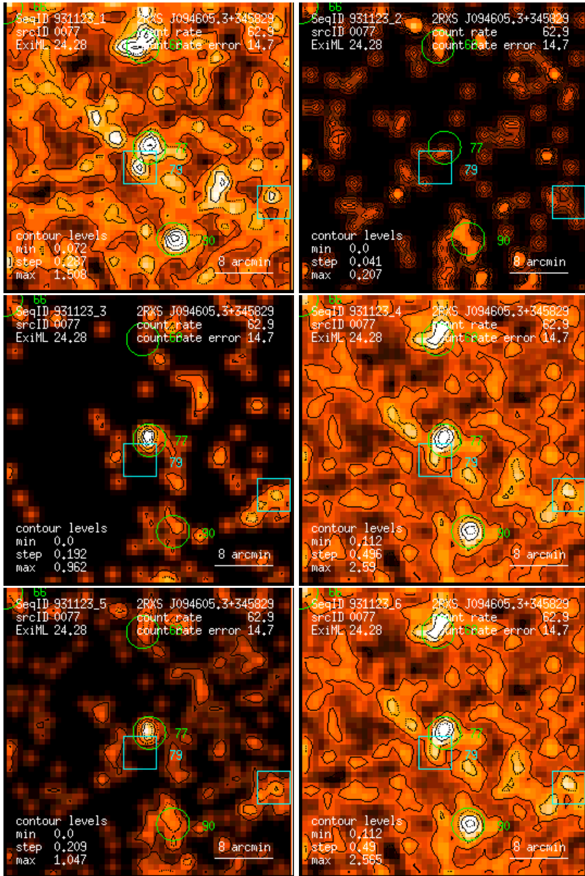
Figure 77: RASS 931123: detection 0077: band rate images, Gaussian filter: (1) PSPC channels 11 – 41, (2) 52 – 90, (3) 91 – 201, (4) 11 – 235, (5) 52 – 201, (6) 11 – 201. Broad band rates in counts/ks. Band rate contour levels in counts/ks/arcmin 2 .
