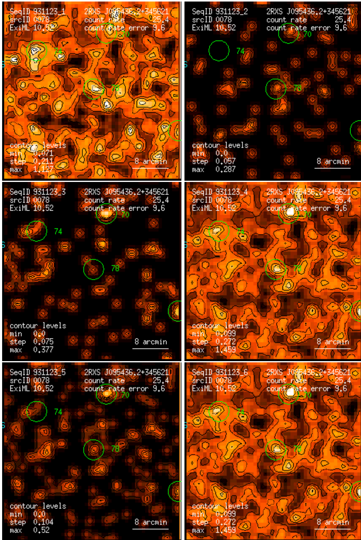
Figure 78: RASS 931123: detection 0078: band rate images, Gaussian filter: (1) PSPC channels 11 – 41, (2) 52 – 90, (3) 91 – 201, (4) 11 – 235, (5) 52 – 201, (6) 11 – 201. Broad band rates in counts/ks. Band rate contour levels in counts/ks/arcmin 2 .
