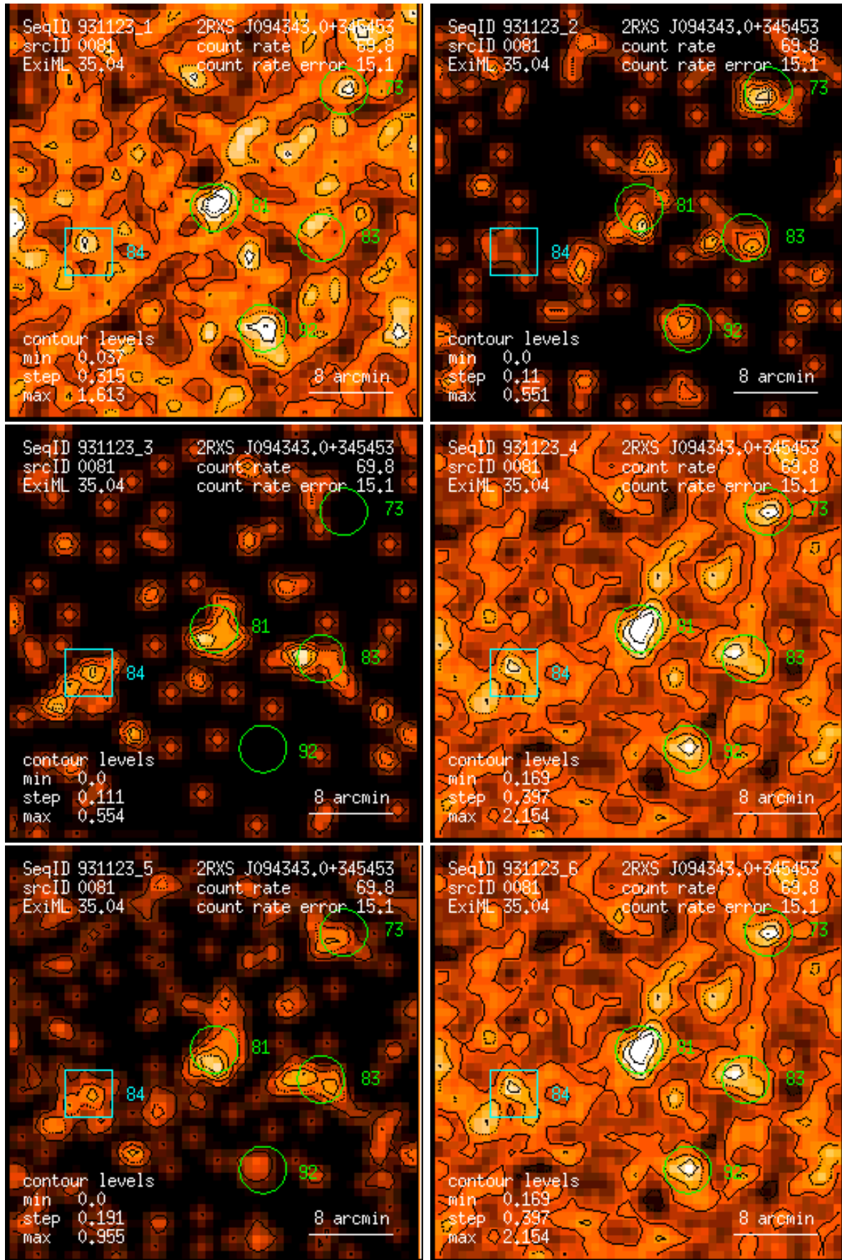
Figure 81: RASS 931123: detection 0081: band rate images, Gaussian filter: (1) PSPC channels 11 – 41, (2) 52 – 90, (3) 91 – 201, (4) 11 – 235, (5) 52 – 201, (6) 11 – 201. Broad band rates in counts/ks. Band rate contour levels in counts/ks/arcmin 2 .
