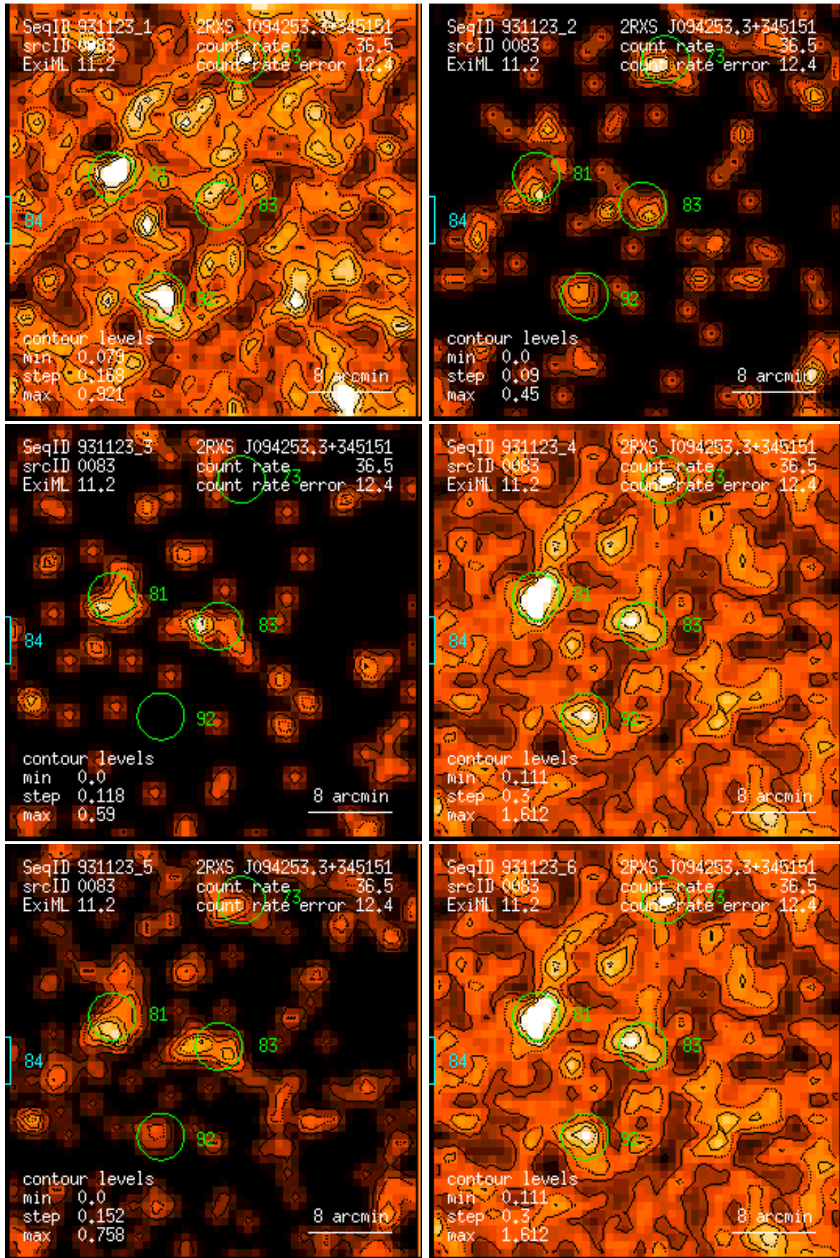
Figure 83: RASS 931123: detection 0083: band rate images, Gaussian filter: (1) PSPC channels 11 – 41, (2) 52 – 90, (3) 91 – 201, (4) 11 – 235, (5) 52 – 201, (6) 11 – 201. Broad band rates in counts/ks. Band rate contour levels in counts/ks/arcmin 2 .
