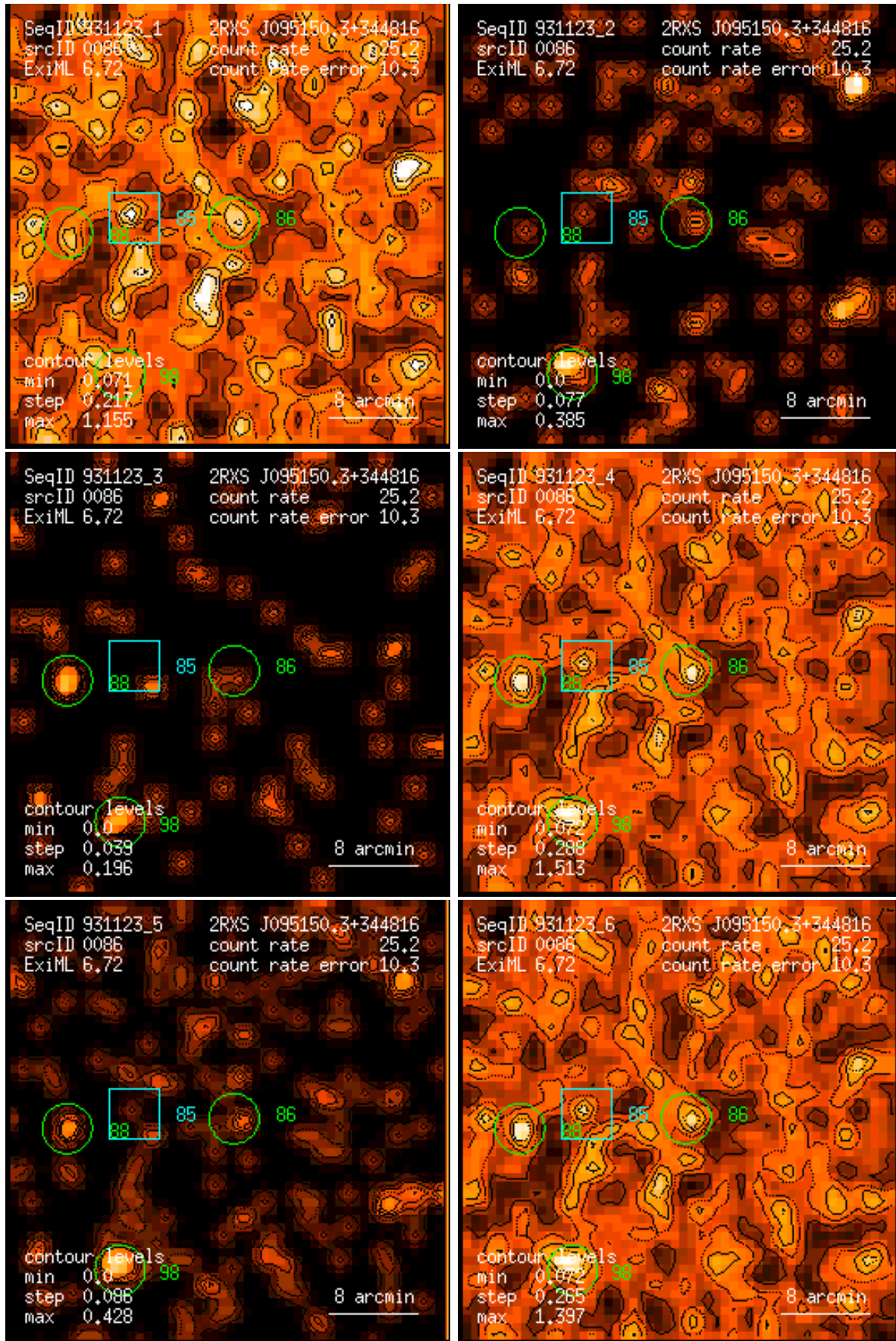
Figure 86: RASS 931123: detection 0086: band rate images, Gaussian filter: (1) PSPC channels 11 – 41, (2) 52 – 90, (3) 91 – 201, (4) 11 – 235, (5) 52 – 201, (6) 11 – 201. Broad band rates in counts/ks. Band rate contour levels in counts/ks/arcmin 2 .
