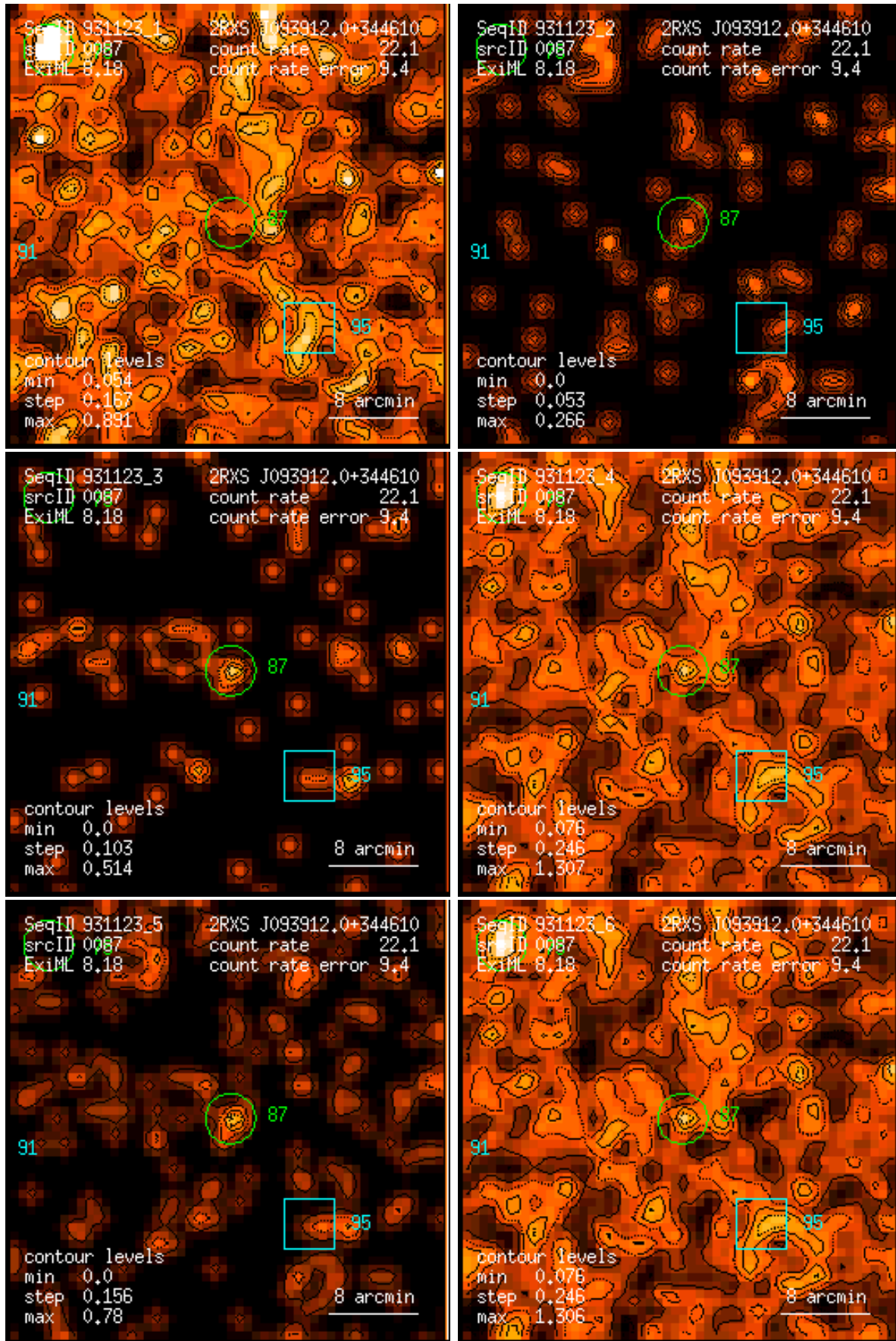
Figure 87: RASS 931123: detection 0087: band rate images, Gaussian filter: (1) PSPC channels 11 – 41, (2) 52 – 90, (3) 91 – 201, (4) 11 – 235, (5) 52 – 201, (6) 11 – 201. Broad band rates in counts/ks. Band rate contour levels in counts/ks/arcmin 2 .
