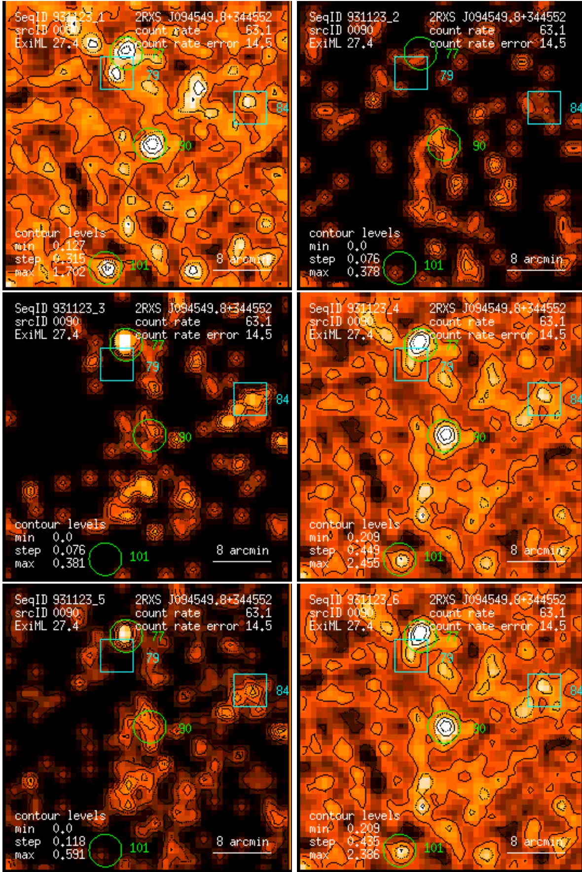
Figure 90: RASS 931123: detection 0090: band rate images, Gaussian filter: (1) PSPC channels 11 – 41, (2) 52 – 90, (3) 91 – 201, (4) 11 – 235, (5) 52 – 201, (6) 11 – 201. Broad band rates in counts/ks. Band rate contour levels in counts/ks/arcmin 2 .
