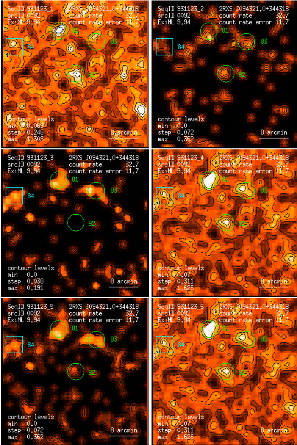
Figure 92: RASS 931123: detection 0092: band rate images, Gaussian filter: (1) PSPC channels 11 – 41, (2) 52 – 90, (3) 91 – 201, (4) 11 – 235, (5) 52 – 201, (6) 11 – 201. Broad band rates in counts/ks. Band rate contour levels in counts/ks/arcmin 2 .
