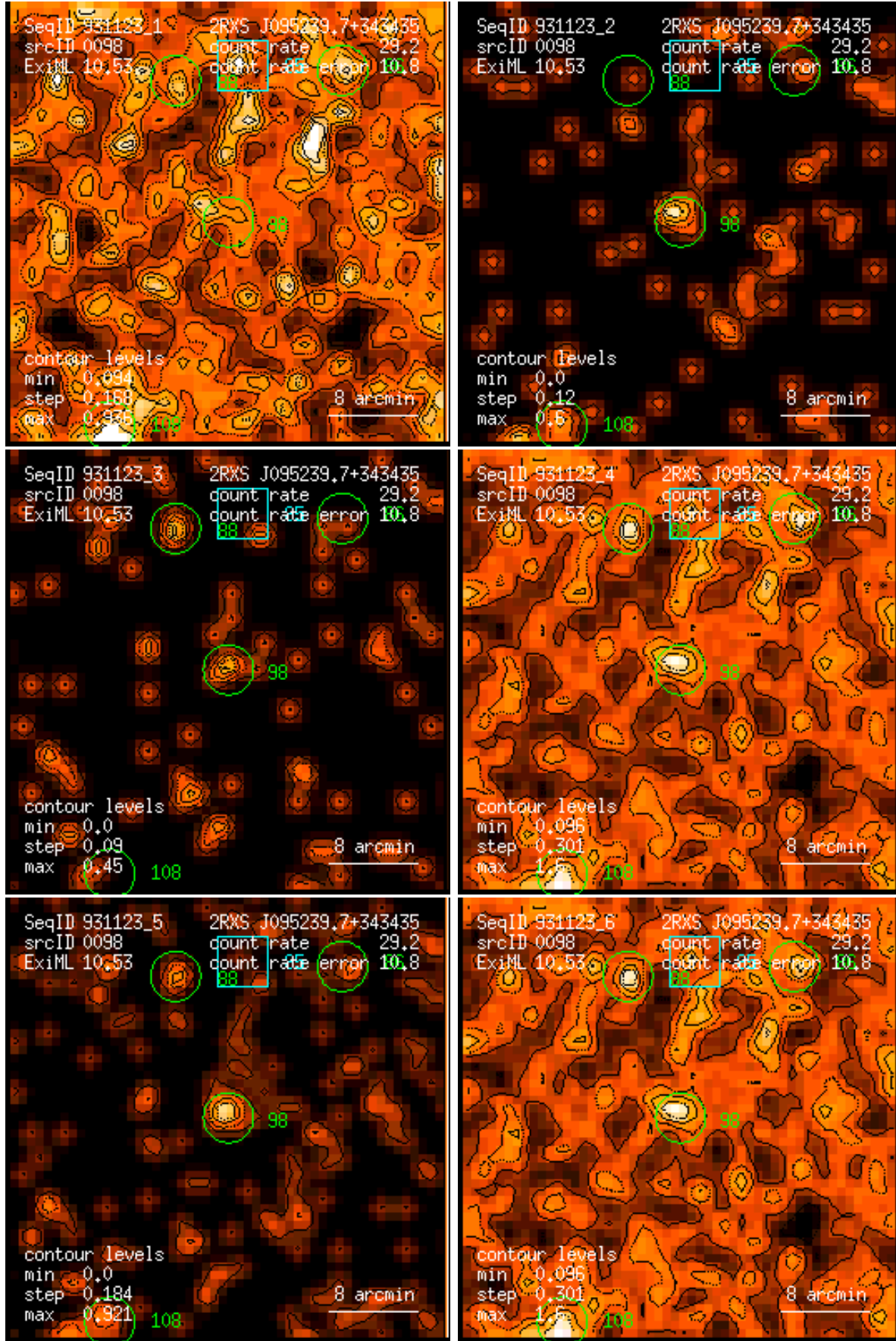
Figure 98: RASS 931123: detection 0098: band rate images, Gaussian filter: (1) PSPC channels 11 – 41, (2) 52 – 90, (3) 91 – 201, (4) 11 – 235, (5) 52 – 201, (6) 11 – 201. Broad band rates in counts/ks. Band rate contour levels in counts/ks/arcmin 2 .
