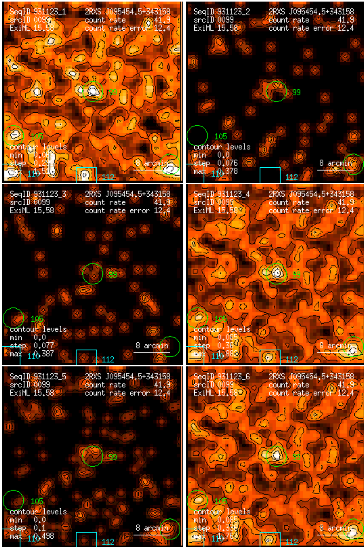
Figure 99: RASS 931123: detection 0099: band rate images, Gaussian filter: (1) PSPC channels 11 – 41, (2) 52 – 90, (3) 91 – 201, (4) 11 – 235, (5) 52 – 201, (6) 11 – 201. Broad band rates in counts/ks. Band rate contour levels in counts/ks/arcmin 2 .
