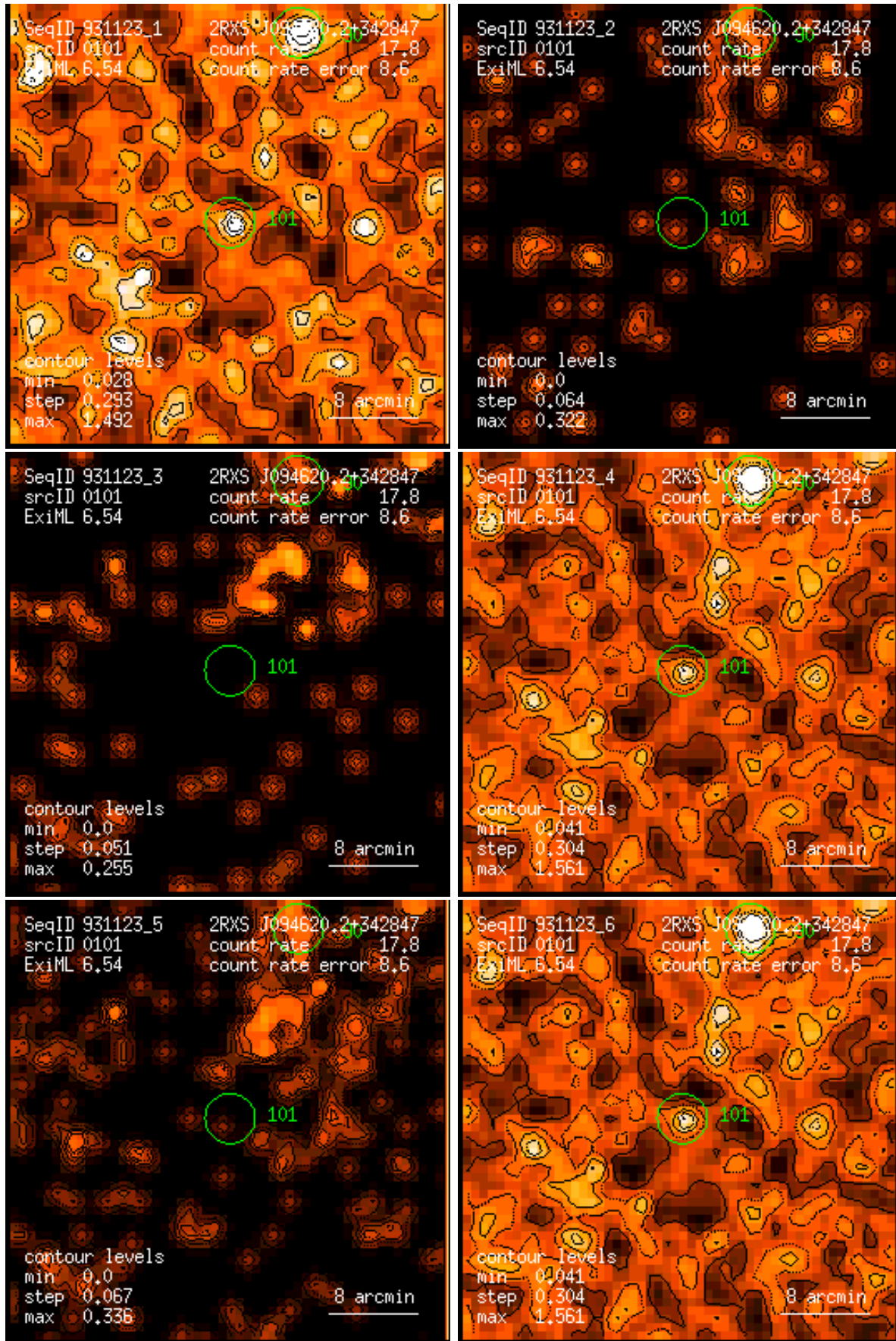
Figure 101: RASS 931123: detection 0101: band rate images, Gaussian filter: (1) PSPC channels 11 – 41, (2) 52 – 90, (3) 91 – 201, (4) 11 – 235, (5) 52 – 201, (6) 11 – 201. Broad band rates in counts/ks. Band rate contour levels in counts/ks/arcmin 2 .
