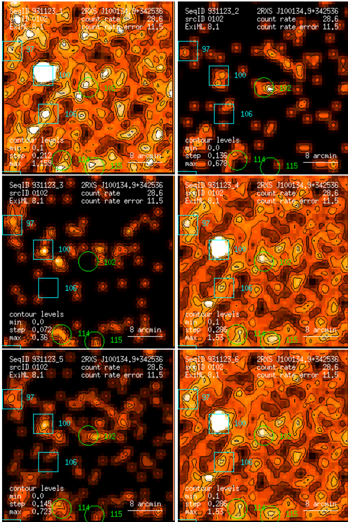
Figure 102: RASS 931123: detection 0102: band rate images, Gaussian filter: (1) PSPC channels 11 – 41, (2) 52 – 90, (3) 91 – 201, (4) 11 – 235, (5) 52 – 201, (6) 11 – 201. Broad band rates in counts/ks. Band rate contour levels in counts/ks/arcmin 2 .
