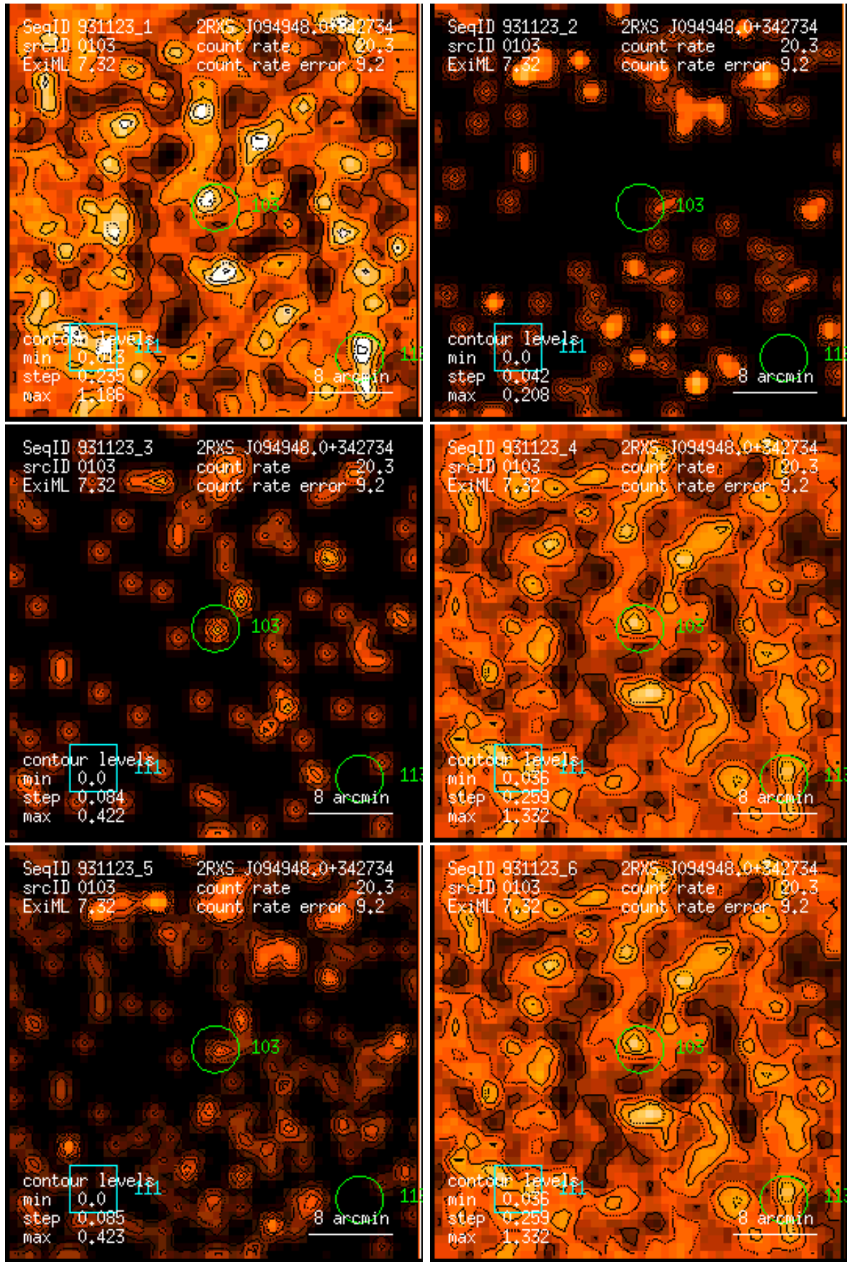
Figure 103: RASS 931123: detection 0103: band rate images, Gaussian filter: (1) PSPC channels 11 – 41, (2) 52 – 90, (3) 91 – 201, (4) 11 – 235, (5) 52 – 201, (6) 11 – 201. Broad band rates in counts/ks. Band rate contour levels in counts/ks/arcmin 2 .
