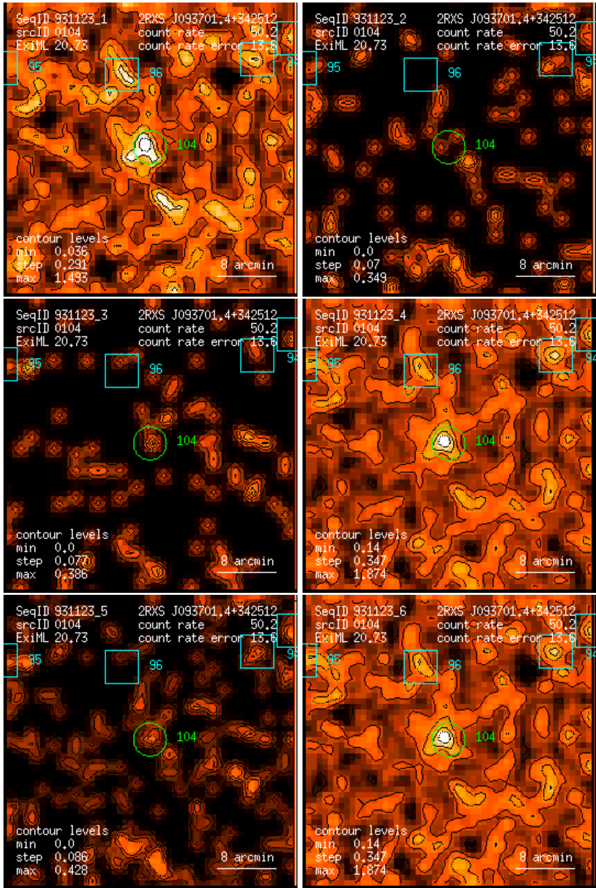
Figure 104: RASS 931123: detection 0104: band rate images, Gaussian filter: (1) PSPC channels 11 – 41, (2) 52 – 90, (3) 91 – 201, (4) 11 – 235, (5) 52 – 201, (6) 11 – 201. Broad band rates in counts/ks. Band rate contour levels in counts/ks/arcmin 2 .
