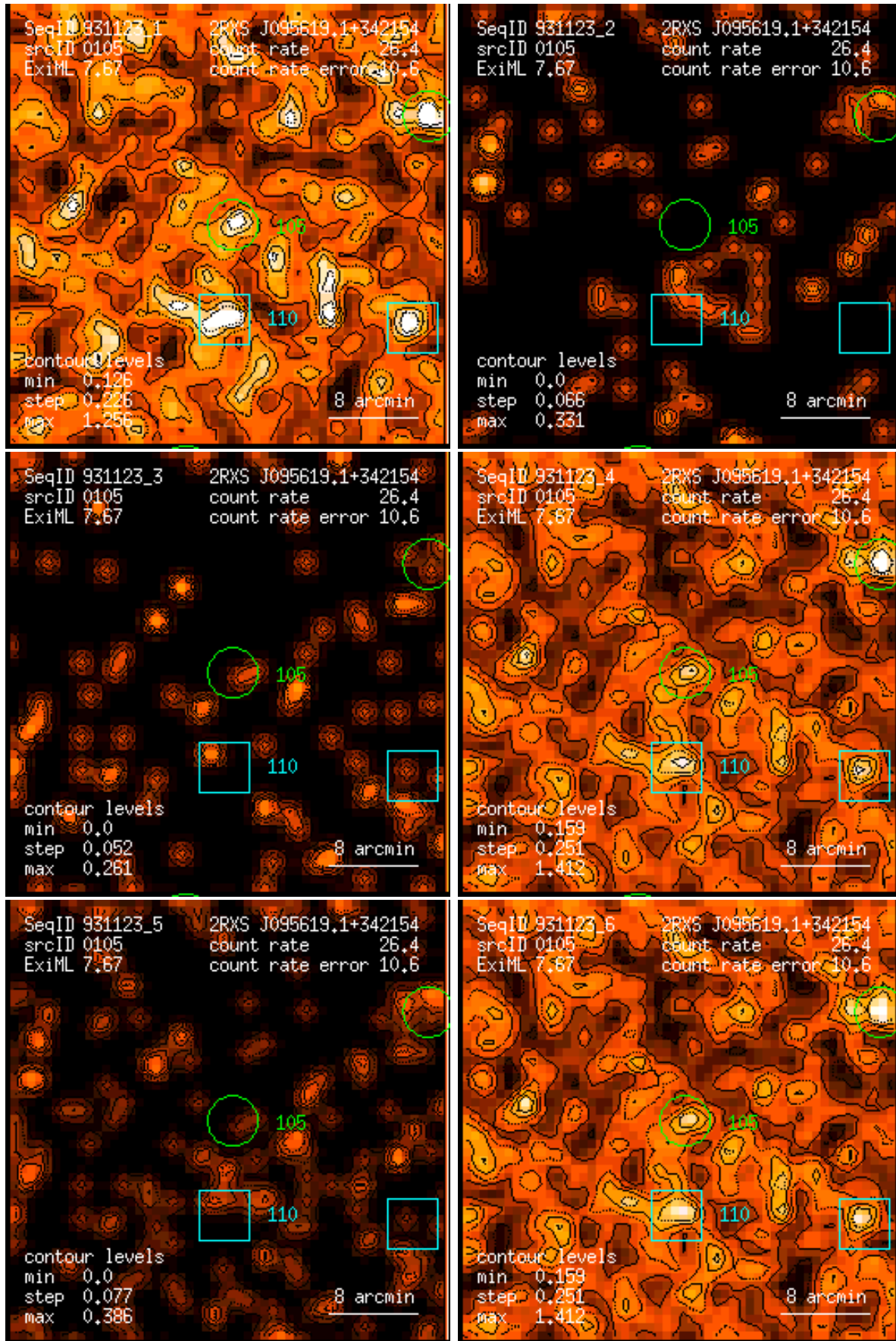
Figure 105: RASS 931123: detection 0105: band rate images, Gaussian filter: (1) PSPC channels 11 – 41, (2) 52 – 90, (3) 91 – 201, (4) 11 – 235, (5) 52 – 201, (6) 11 – 201. Broad band rates in counts/ks. Band rate contour levels in counts/ks/arcmin 2 .
