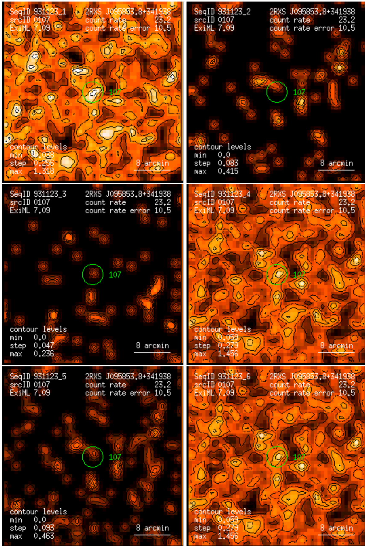
Figure 107: RASS 931123: detection 0107: band rate images, Gaussian filter: (1) PSPC channels 11 – 41, (2) 52 – 90, (3) 91 – 201, (4) 11 – 235, (5) 52 – 201, (6) 11 – 201. Broad band rates in counts/ks. Band rate contour levels in counts/ks/arcmin 2 .
