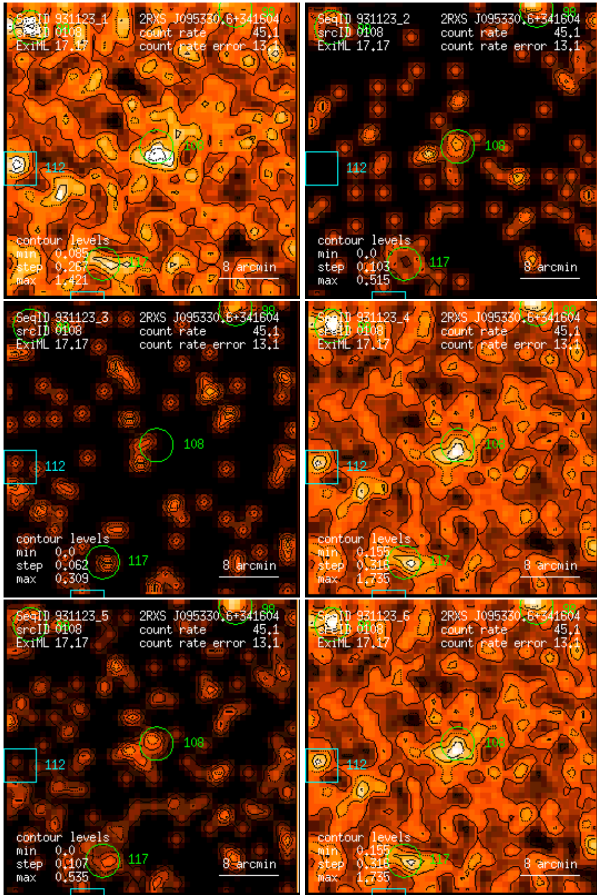
Figure 108: RASS 931123: detection 0108: band rate images, Gaussian filter: (1) PSPC channels 11 – 41, (2) 52 – 90, (3) 91 – 201, (4) 11 – 235, (5) 52 – 201, (6) 11 – 201. Broad band rates in counts/ks. Band rate contour levels in counts/ks/arcmin 2 .
