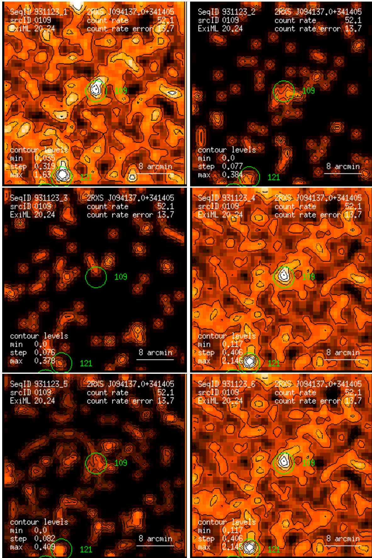
Figure 109: RASS 931123: detection 0109: band rate images, Gaussian filter: (1) PSPC channels 11 – 41, (2) 52 – 90, (3) 91 – 201, (4) 11 – 235, (5) 52 – 201, (6) 11 – 201. Broad band rates in counts/ks. Band rate contour levels in counts/ks/arcmin 2 .
