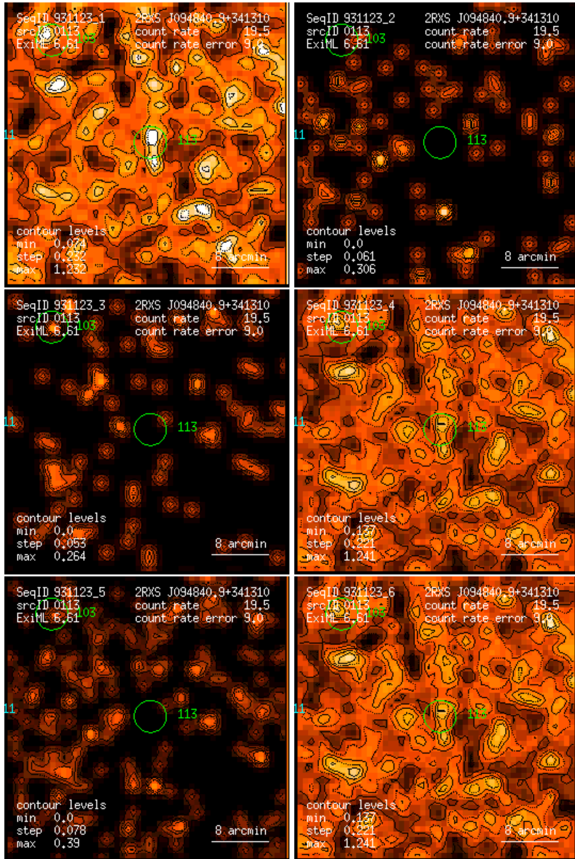
Figure 113: RASS 931123: detection 0113: band rate images, Gaussian filter: (1) PSPC channels 11 – 41, (2) 52 – 90, (3) 91 – 201, (4) 11 – 235, (5) 52 – 201, (6) 11 – 201. Broad band rates in counts/ks. Band rate contour levels in counts/ks/arcmin 2 .
