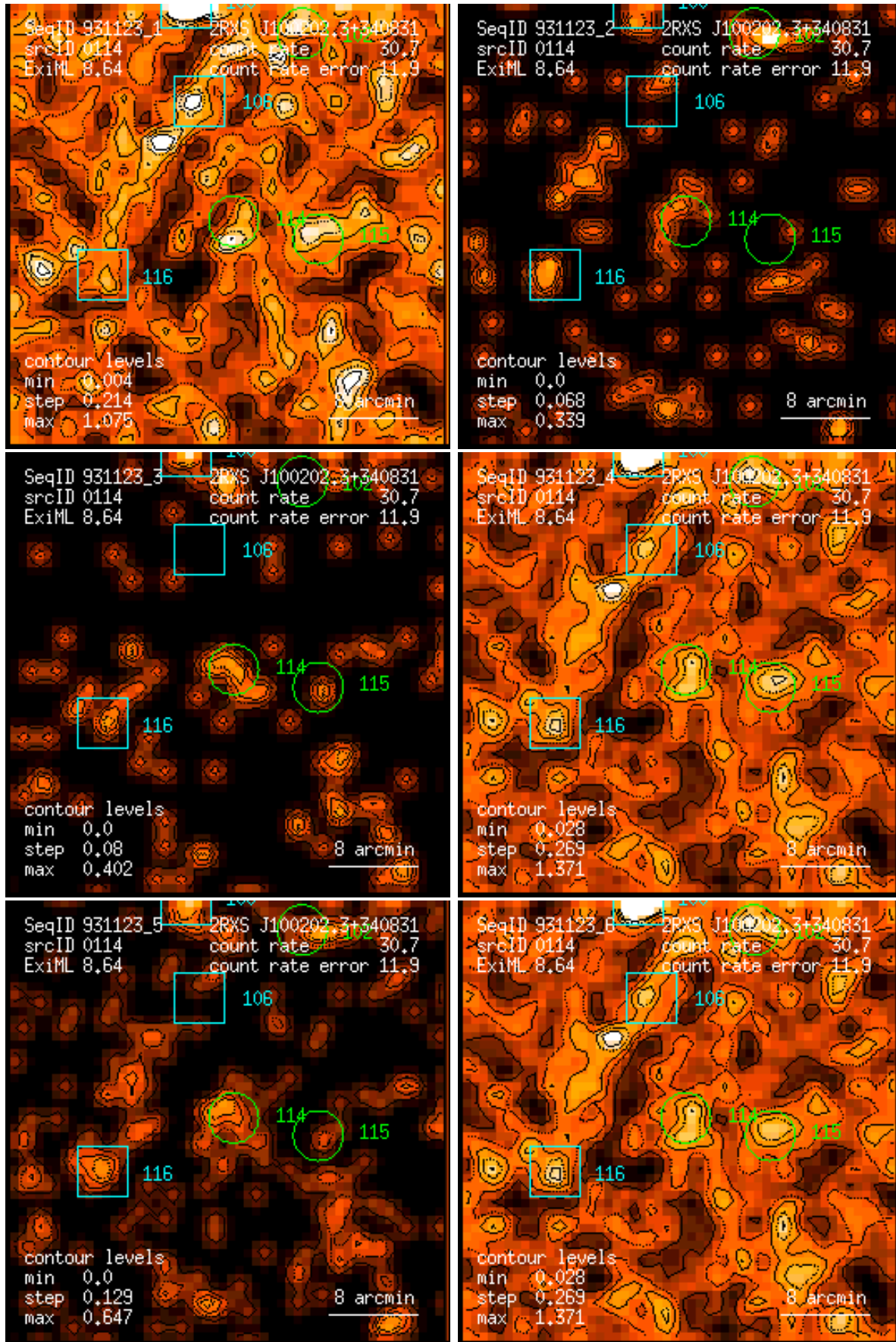
Figure 114: RASS 931123: detection 0114: band rate images, Gaussian filter: (1) PSPC channels 11 – 41, (2) 52 – 90, (3) 91 – 201, (4) 11 – 235, (5) 52 – 201, (6) 11 – 201. Broad band rates in counts/ks. Band rate contour levels in counts/ks/arcmin 2 .
