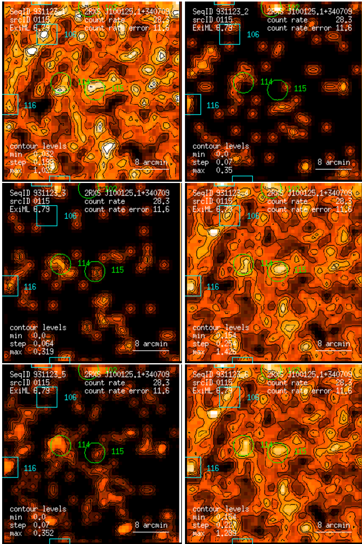
Figure 115: RASS 931123: detection 0115: band rate images, Gaussian filter: (1) PSPC channels 11 – 41, (2) 52 – 90, (3) 91 – 201, (4) 11 – 235, (5) 52 – 201, (6) 11 – 201. Broad band rates in counts/ks. Band rate contour levels in counts/ks/arcmin 2 .
