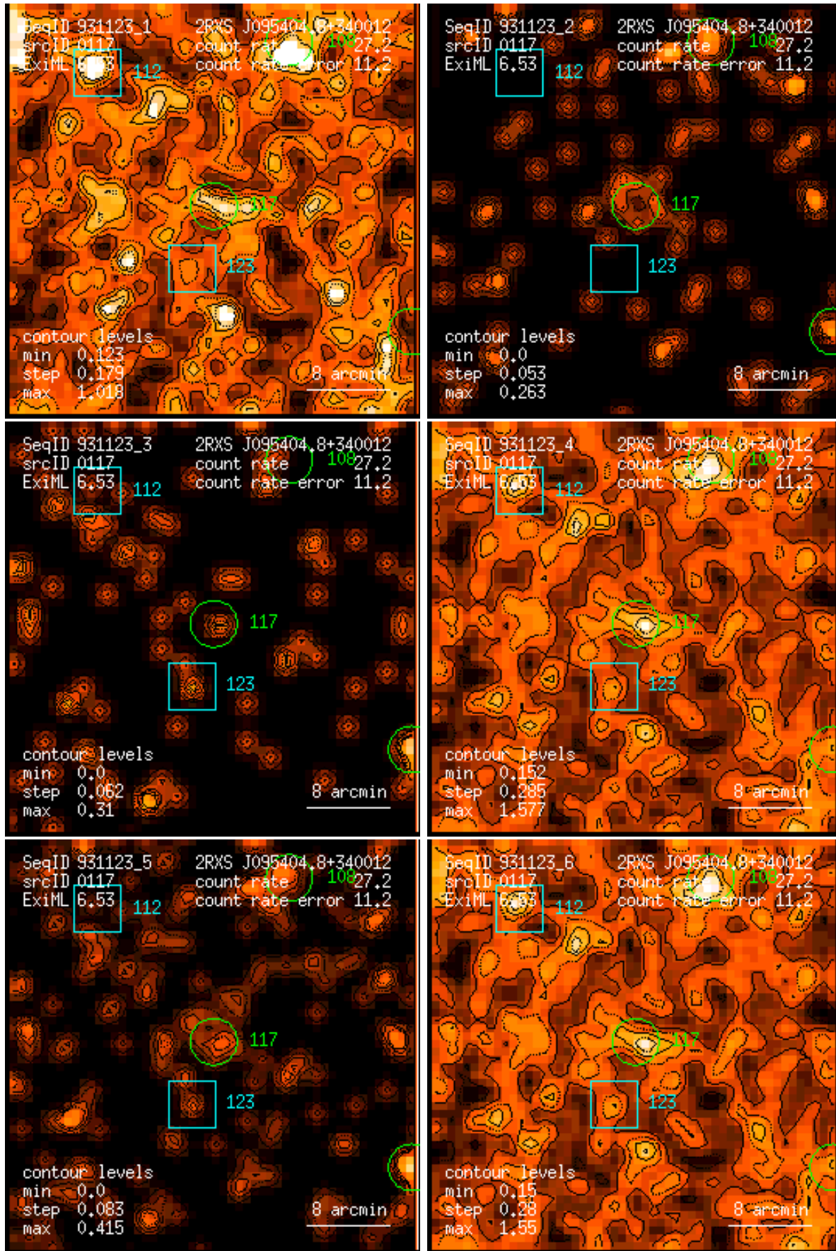
Figure 117: RASS 931123: detection 0117: band rate images, Gaussian filter: (1) PSPC channels 11 – 41, (2) 52 – 90, (3) 91 – 201, (4) 11 – 235, (5) 52 – 201, (6) 11 – 201. Broad band rates in counts/ks. Band rate contour levels in counts/ks/arcmin 2 .
