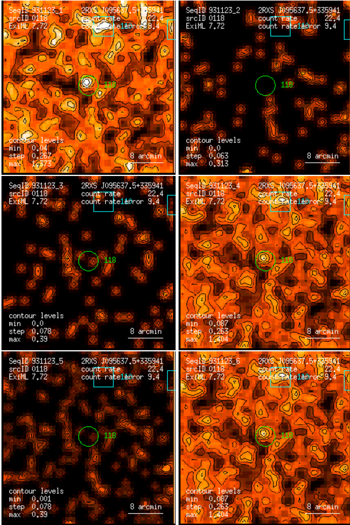
Figure 118: RASS 931123: detection 0118: band rate images, Gaussian filter: (1) PSPC channels 11 – 41, (2) 52 – 90, (3) 91 – 201, (4) 11 – 235, (5) 52 – 201, (6) 11 – 201. Broad band rates in counts/ks. Band rate contour levels in counts/ks/arcmin 2 .
