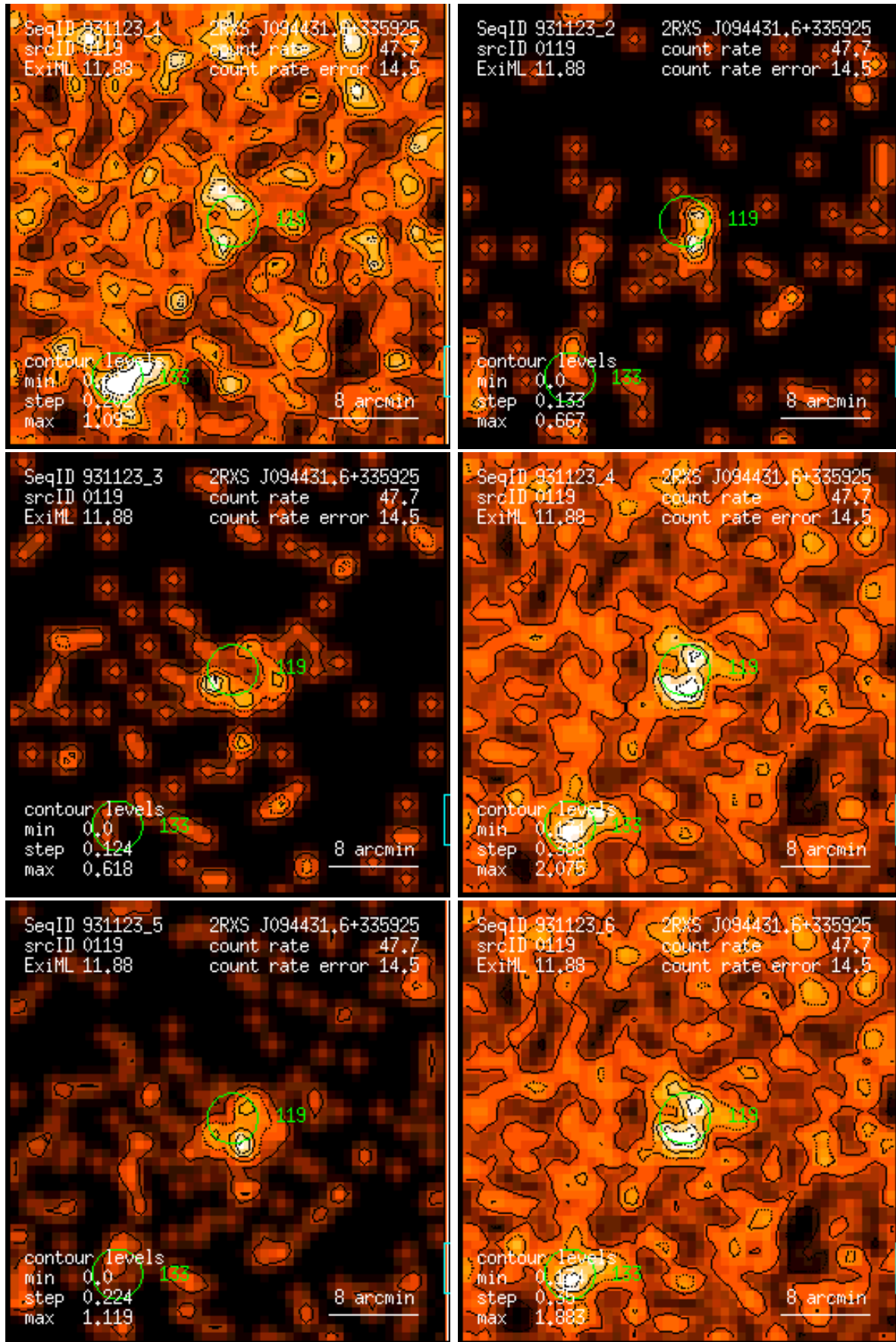
Figure 119: RASS 931123: detection 0119: band rate images, Gaussian filter: (1) PSPC channels 11 – 41, (2) 52 – 90, (3) 91 – 201, (4) 11 – 235, (5) 52 – 201, (6) 11 – 201. Broad band rates in counts/ks. Band rate contour levels in counts/ks/arcmin 2 .
