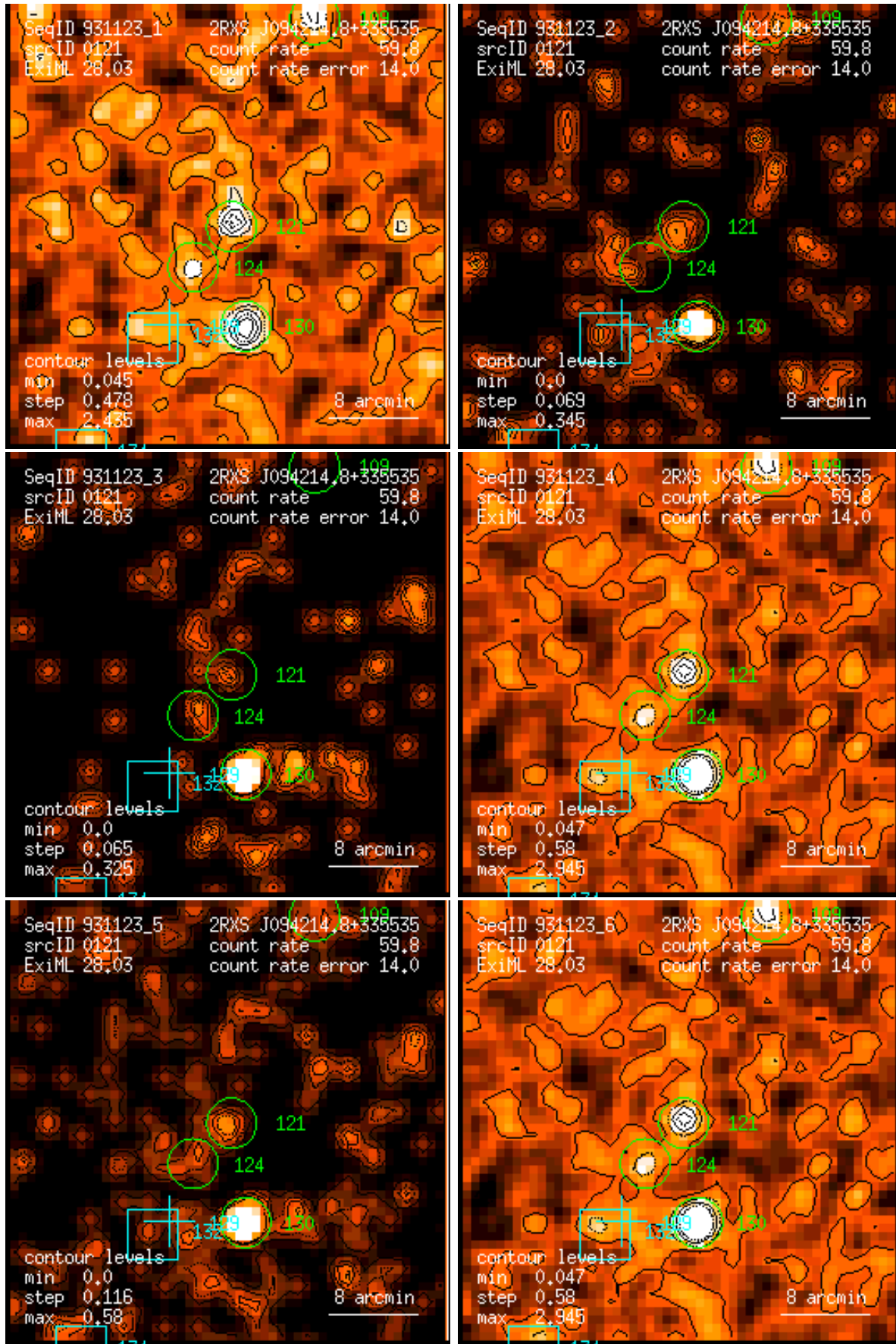
Figure 121: RASS 931123: detection 0121: band rate images, Gaussian filter: (1) PSPC channels 11 – 41, (2) 52 – 90, (3) 91 – 201, (4) 11 – 235, (5) 52 – 201, (6) 11 – 201. Broad band rates in counts/ks. Band rate contour levels in counts/ks/arcmin 2 .
