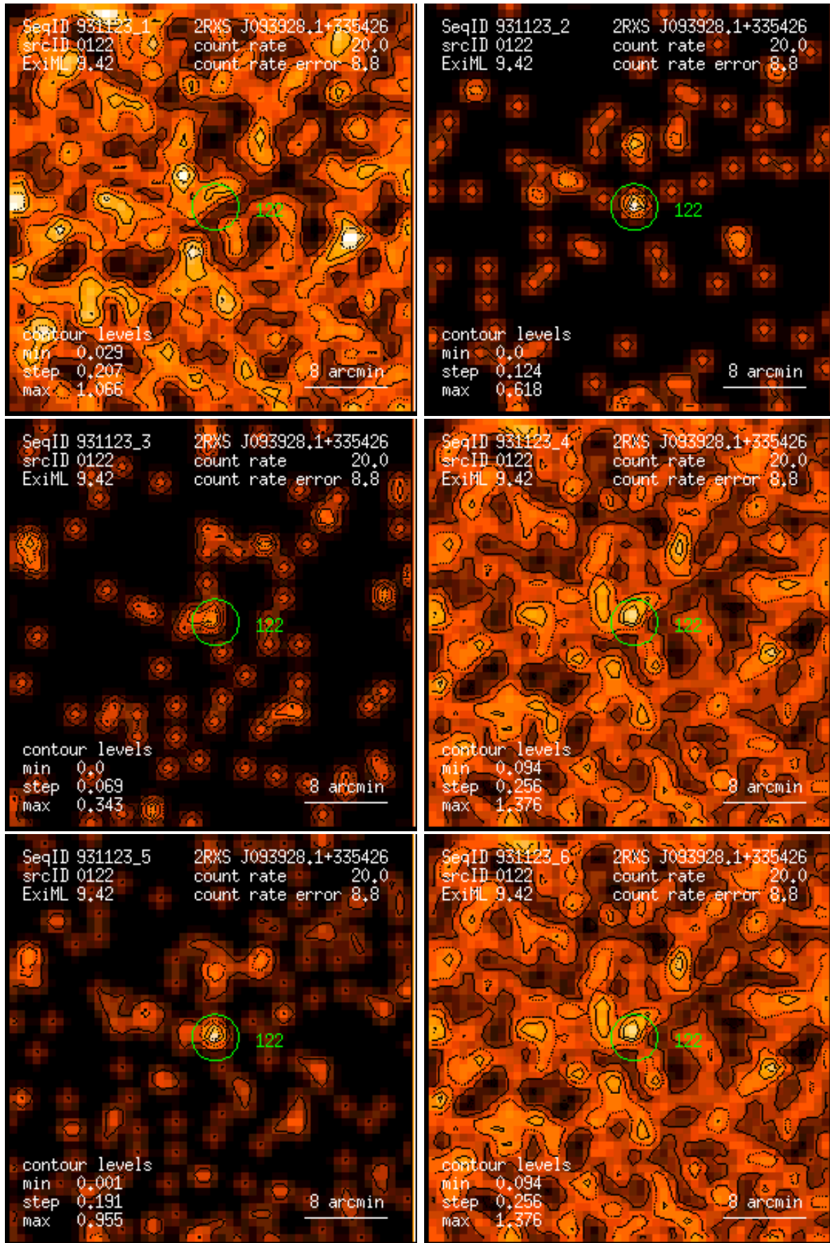
Figure 122: RASS 931123: detection 0122: band rate images, Gaussian filter: (1) PSPC channels 11 – 41, (2) 52 – 90, (3) 91 – 201, (4) 11 – 235, (5) 52 – 201, (6) 11 – 201. Broad band rates in counts/ks. Band rate contour levels in counts/ks/arcmin 2 .
