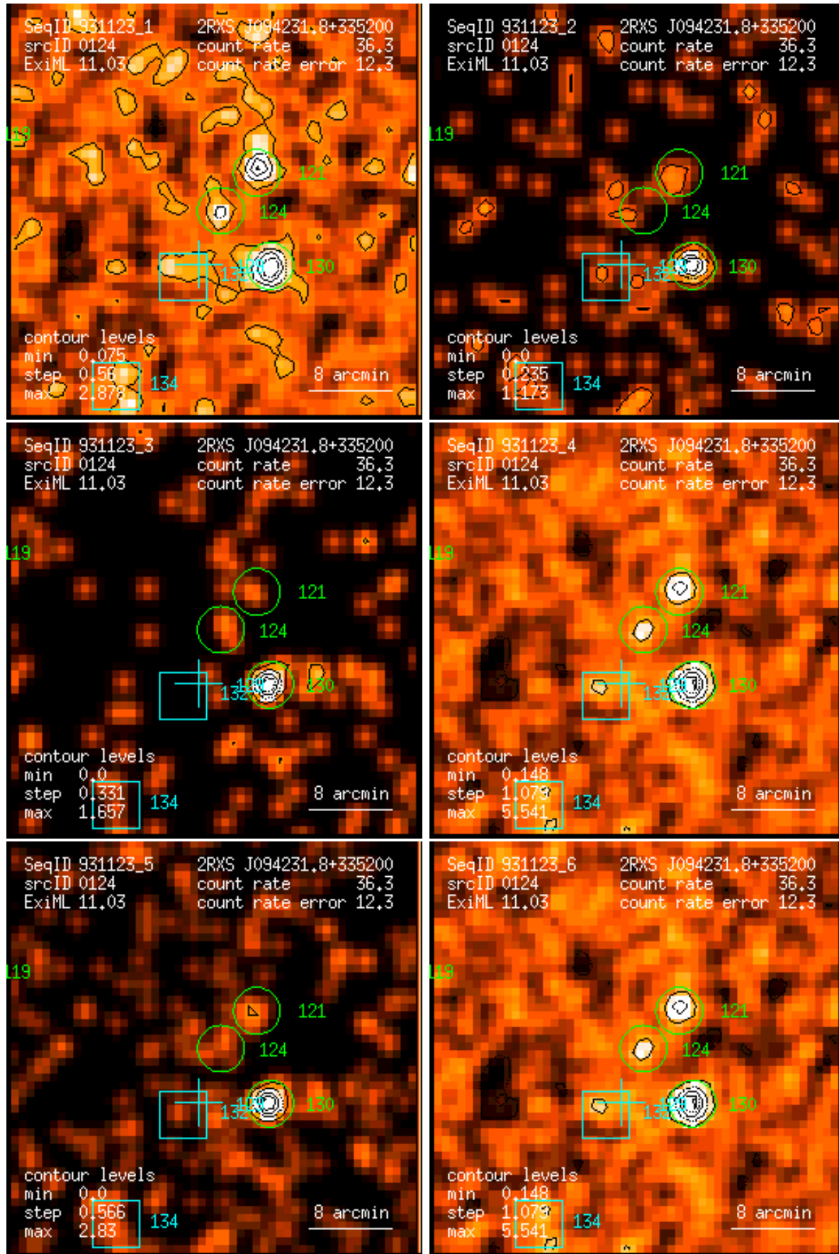
Figure 124: RASS 931123: detection 0124: band rate images, Gaussian filter: (1) PSPC channels 11 – 41, (2) 52 – 90, (3) 91 – 201, (4) 11 – 235, (5) 52 – 201, (6) 11 – 201. Broad band rates in counts/ks. Band rate contour levels in counts/ks/arcmin 2 .
