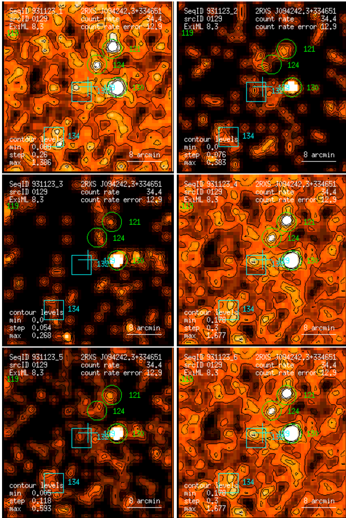
Figure 129: RASS 931123: detection 0129: band rate images, Gaussian filter: (1) PSPC channels 11 – 41, (2) 52 – 90, (3) 91 – 201, (4) 11 – 235, (5) 52 – 201, (6) 11 – 201. Broad band rates in counts/ks. Band rate contour levels in counts/ks/arcmin 2 .
