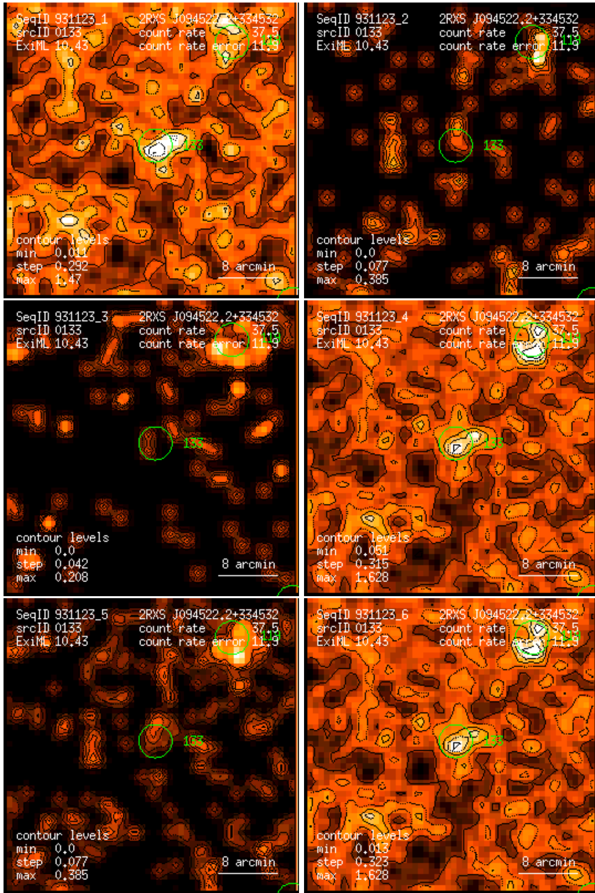
Figure 133: RASS 931123: detection 0133: band rate images, Gaussian filter: (1) PSPC channels 11 – 41, (2) 52 – 90, (3) 91 – 201, (4) 11 – 235, (5) 52 – 201, (6) 11 – 201. Broad band rates in counts/ks. Band rate contour levels in counts/ks/arcmin 2 .
