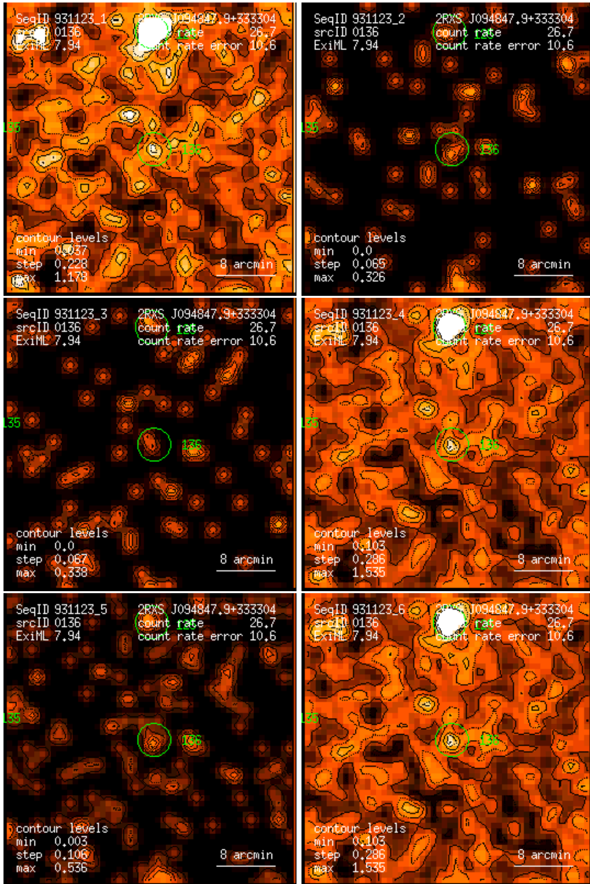
Figure 136: RASS 931123: detection 0136: band rate images, Gaussian filter: (1) PSPC channels 11 – 41, (2) 52 – 90, (3) 91 – 201, (4) 11 – 235, (5) 52 – 201, (6) 11 – 201. Broad band rates in counts/ks. Band rate contour levels in counts/ks/arcmin 2 .
