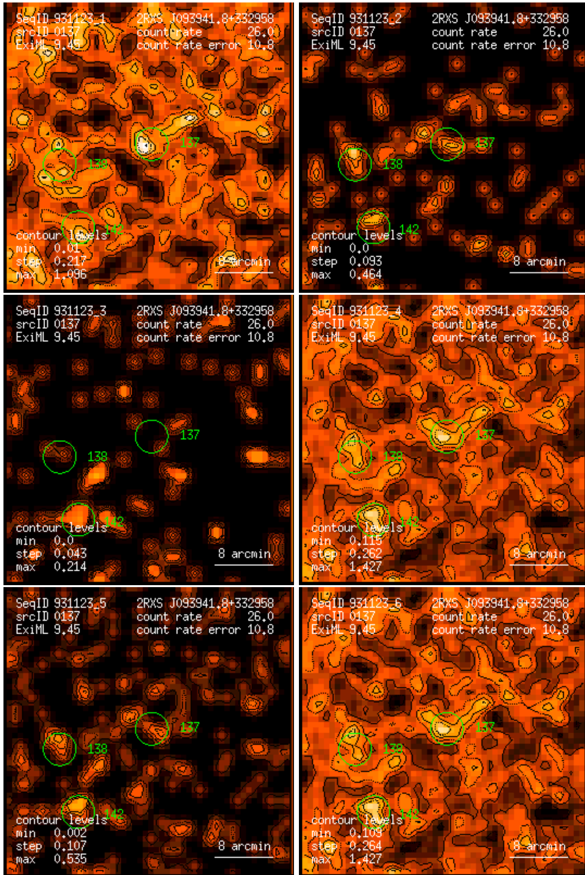
Figure 137: RASS 931123: detection 0137: band rate images, Gaussian filter: (1) PSPC channels 11 – 41, (2) 52 – 90, (3) 91 – 201, (4) 11 – 235, (5) 52 – 201, (6) 11 – 201. Broad band rates in counts/ks. Band rate contour levels in counts/ks/arcmin 2 .
