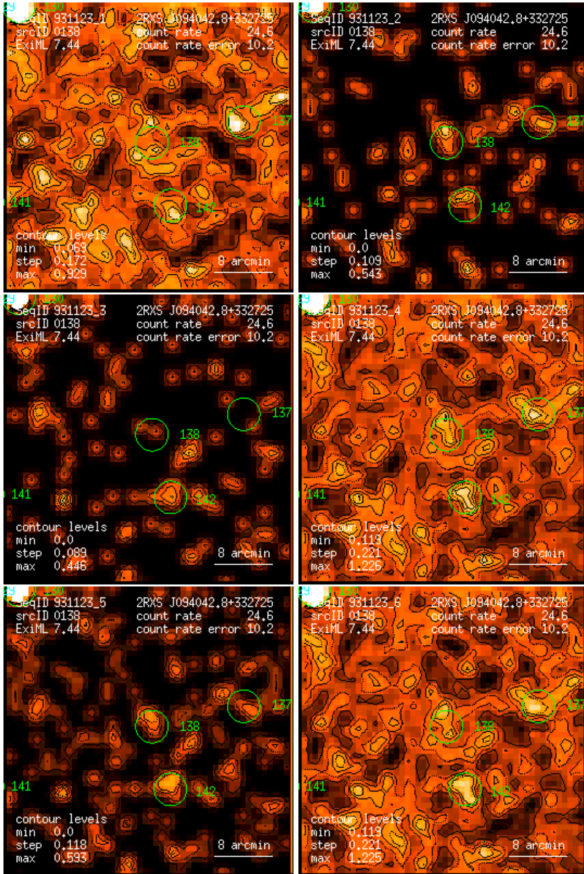
Figure 138: RASS 931123: detection 0138: band rate images, Gaussian filter: (1) PSPC channels 11 – 41, (2) 52 – 90, (3) 91 – 201, (4) 11 – 235, (5) 52 – 201, (6) 11 – 201. Broad band rates in counts/ks. Band rate contour levels in counts/ks/arcmin 2 .
