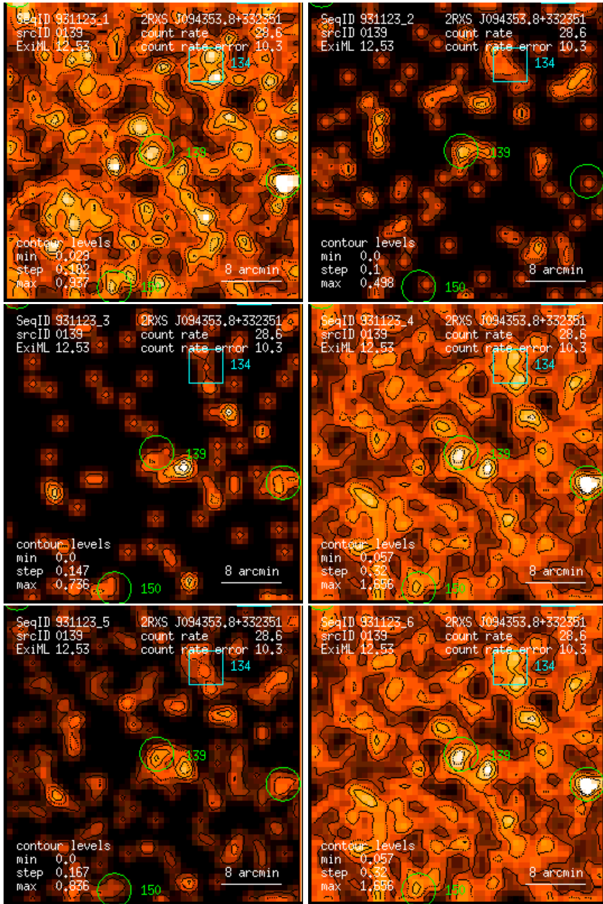
Figure 139: RASS 931123: detection 0139: band rate images, Gaussian filter: (1) PSPC channels 11 – 41, (2) 52 – 90, (3) 91 – 201, (4) 11 – 235, (5) 52 – 201, (6) 11 – 201. Broad band rates in counts/ks. Band rate contour levels in counts/ks/arcmin 2 .
