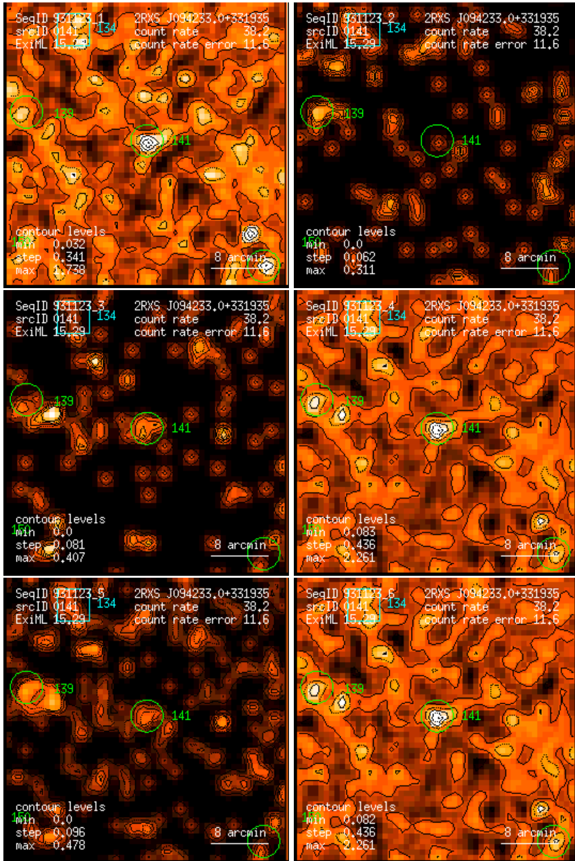
Figure 141: RASS 931123: detection 0141: band rate images, Gaussian filter: (1) PSPC channels 11 – 41, (2) 52 – 90, (3) 91 – 201, (4) 11 – 235, (5) 52 – 201, (6) 11 – 201. Broad band rates in counts/ks. Band rate contour levels in counts/ks/arcmin 2 .
