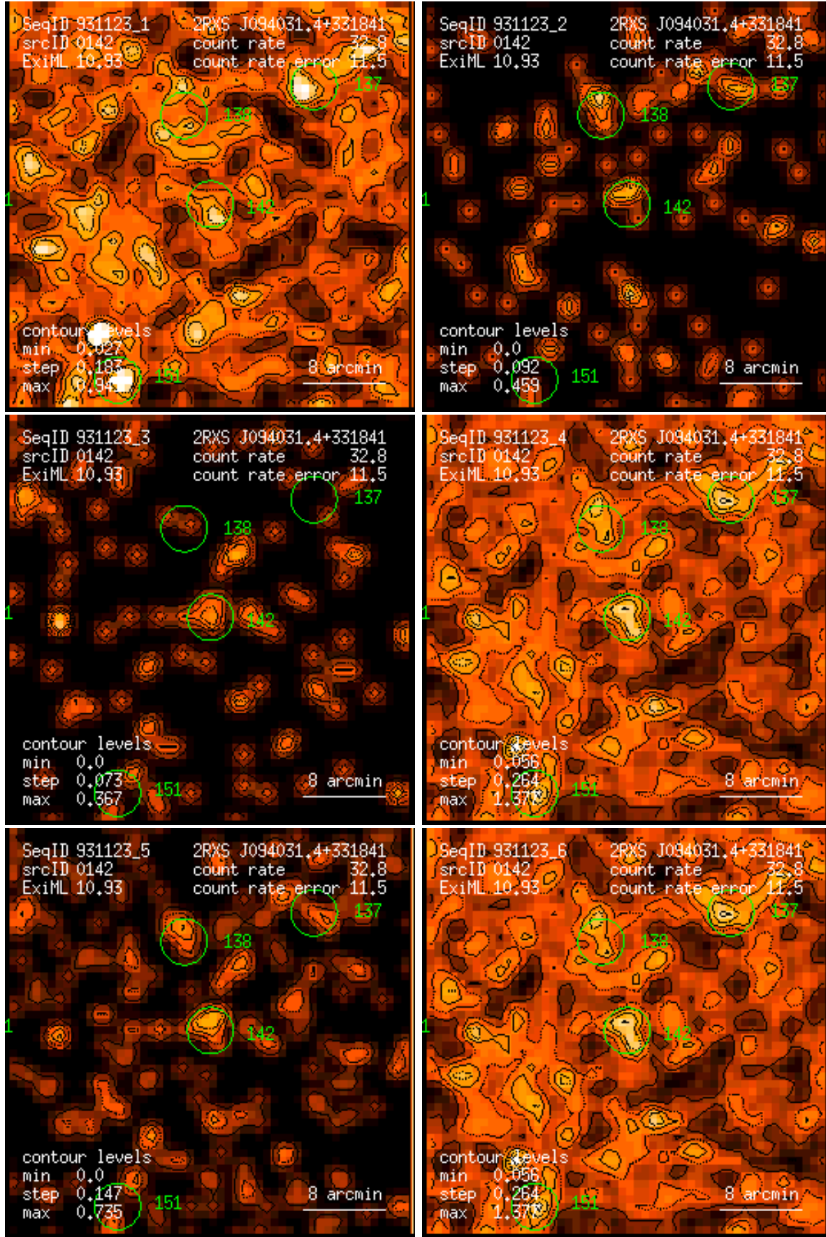
Figure 142: RASS 931123: detection 0142: band rate images, Gaussian filter: (1) PSPC channels 11 – 41, (2) 52 – 90, (3) 91 – 201, (4) 11 – 235, (5) 52 – 201, (6) 11 – 201. Broad band rates in counts/ks. Band rate contour levels in counts/ks/arcmin 2 .
