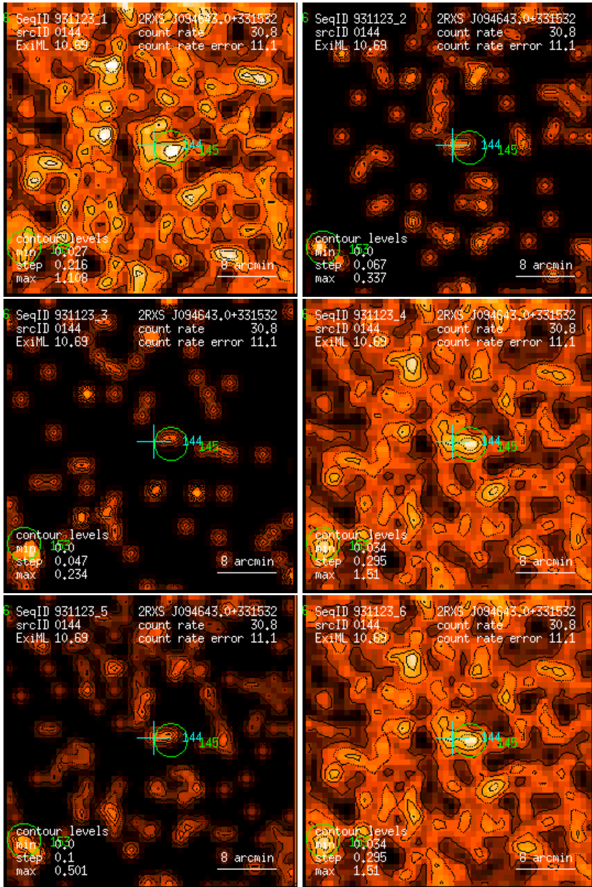
Figure 144: RASS 931123: detection 0144: band rate images, Gaussian filter: (1) PSPC channels 11 – 41, (2) 52 – 90, (3) 91 – 201, (4) 11 – 235, (5) 52 – 201, (6) 11 – 201. Broad band rates in counts/ks. Band rate contour levels in counts/ks/arcmin 2 .
