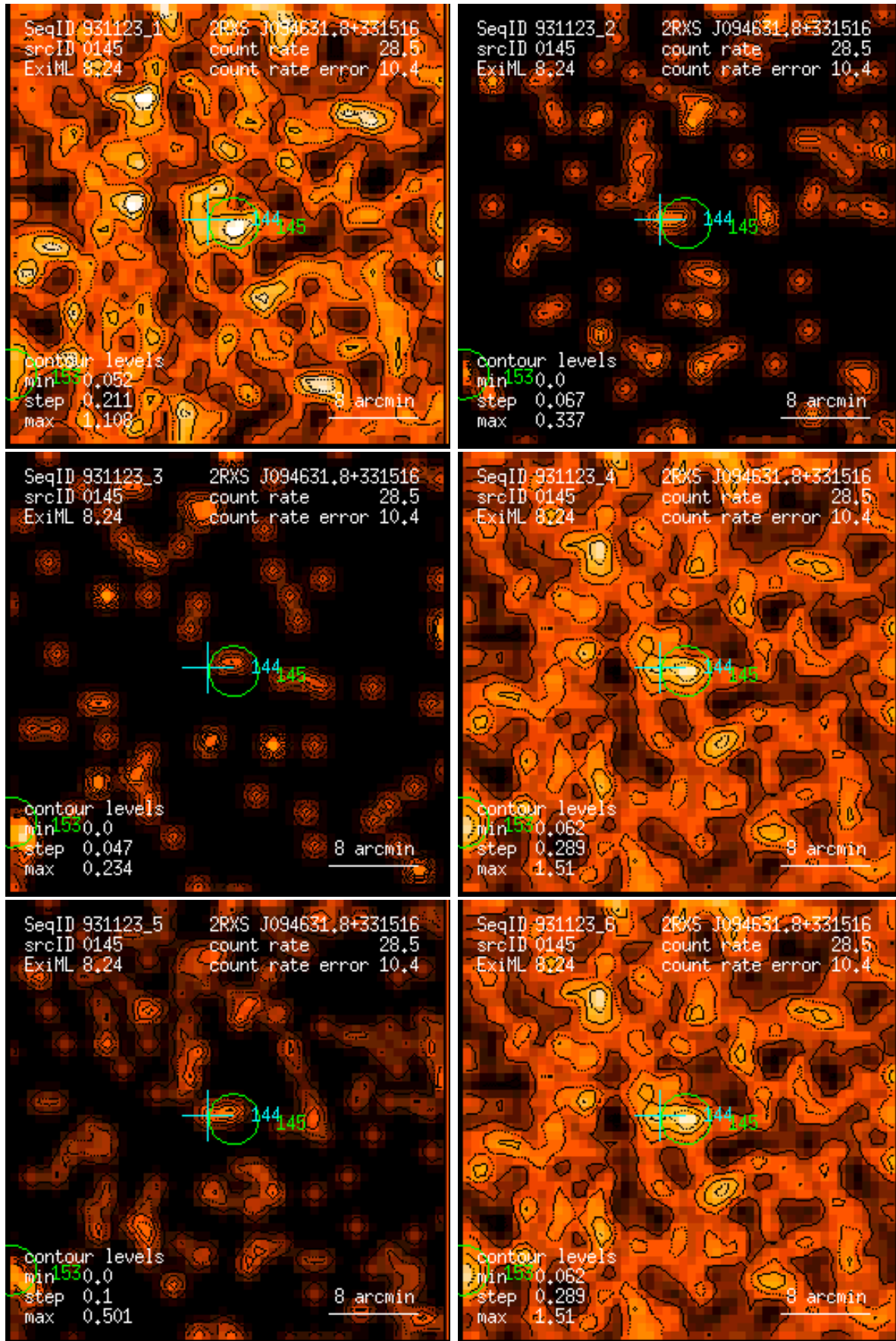
Figure 145: RASS 931123: detection 0145: band rate images, Gaussian filter: (1) PSPC channels 11 – 41, (2) 52 – 90, (3) 91 – 201, (4) 11 – 235, (5) 52 – 201, (6) 11 – 201. Broad band rates in counts/ks. Band rate contour levels in counts/ks/arcmin 2 .
