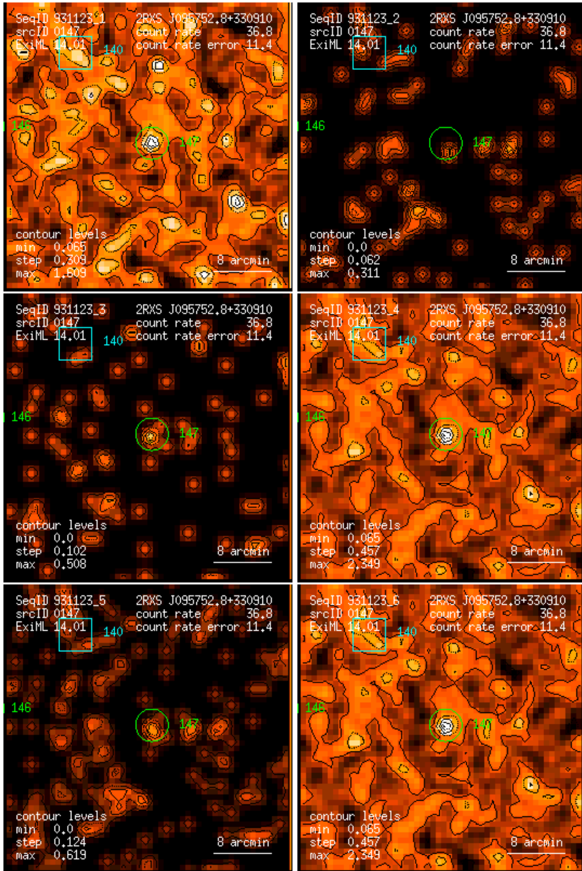
Figure 147: RASS 931123: detection 0147: band rate images, Gaussian filter: (1) PSPC channels 11 – 41, (2) 52 – 90, (3) 91 – 201, (4) 11 – 235, (5) 52 – 201, (6) 11 – 201. Broad band rates in counts/ks. Band rate contour levels in counts/ks/arcmin 2 .
