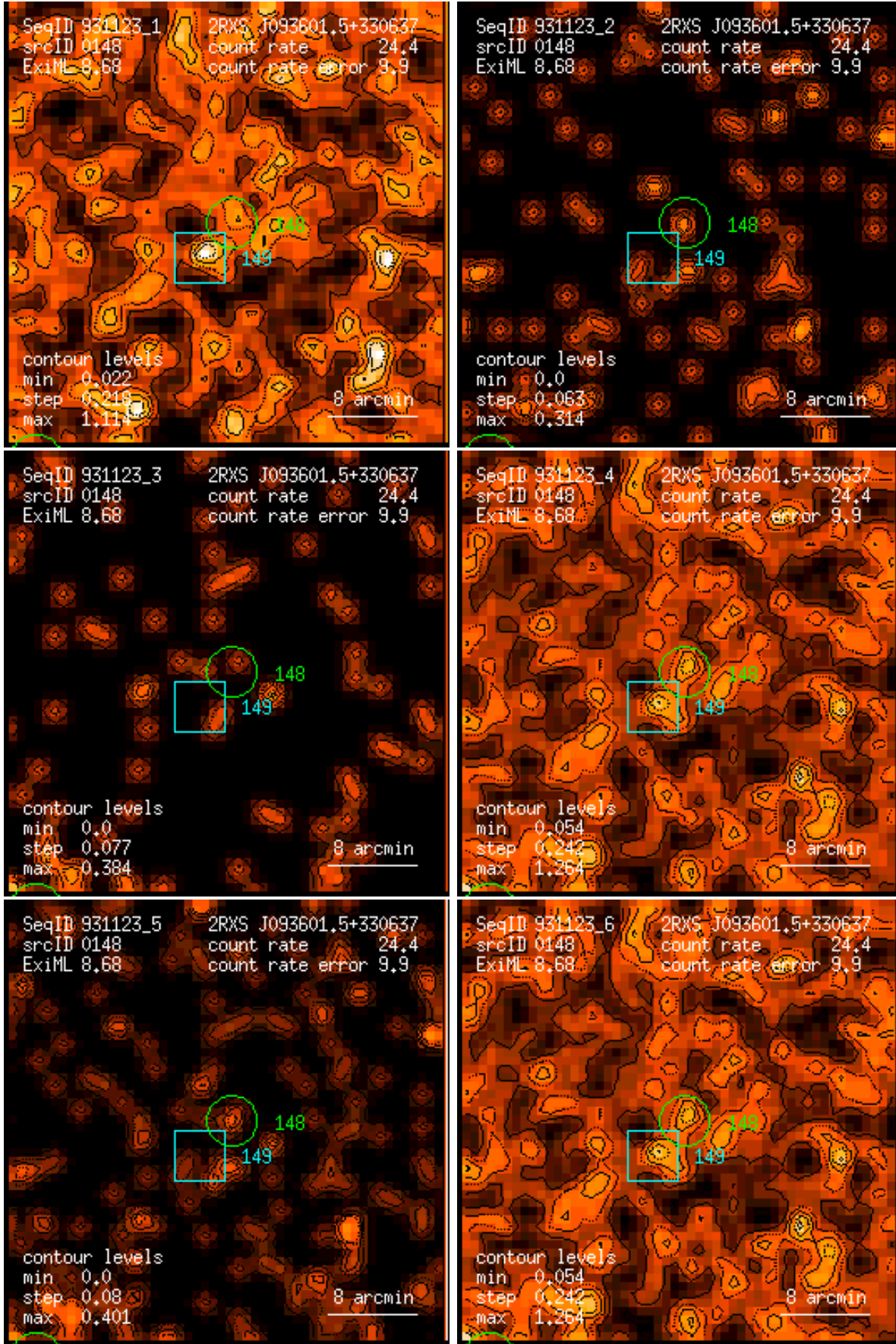
Figure 148: RASS 931123: detection 0148: band rate images, Gaussian filter: (1) PSPC channels 11 – 41, (2) 52 – 90, (3) 91 – 201, (4) 11 – 235, (5) 52 – 201, (6) 11 – 201. Broad band rates in counts/ks. Band rate contour levels in counts/ks/arcmin 2 .
