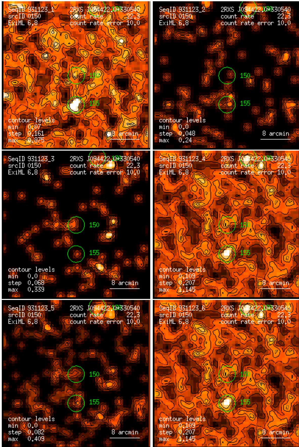
Figure 150: RASS 931123: detection 0150: band rate images, Gaussian filter: (1) PSPC channels 11 – 41, (2) 52 – 90, (3) 91 – 201, (4) 11 – 235, (5) 52 – 201, (6) 11 – 201. Broad band rates in counts/ks. Band rate contour levels in counts/ks/arcmin 2 .
